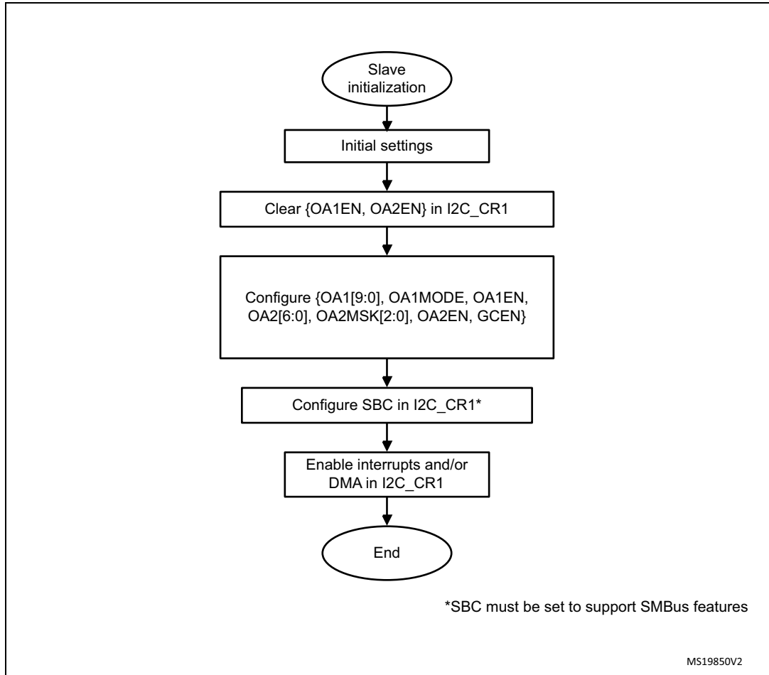
Figure 208. Slave initialization flowchart
