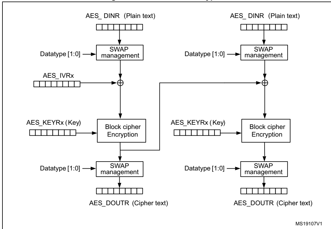
Figure 84. CBC mode encryption
