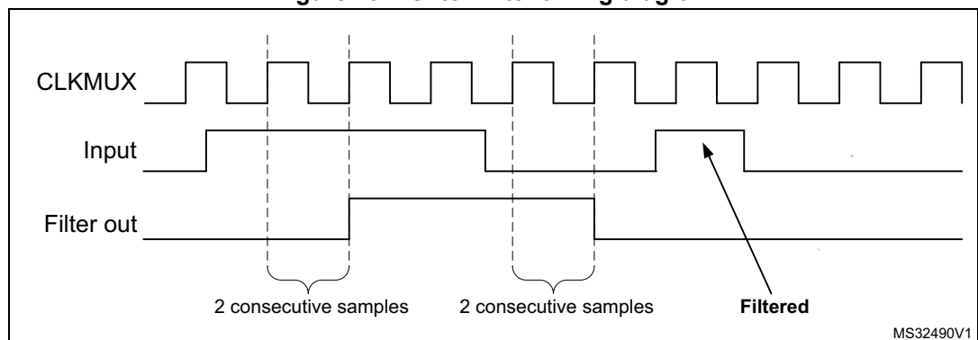
Figure 194. Glitch filter timing diagram
