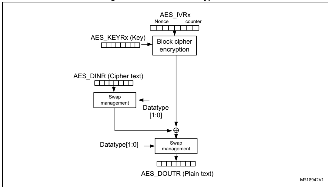
Figure 88. CTR mode decryption
