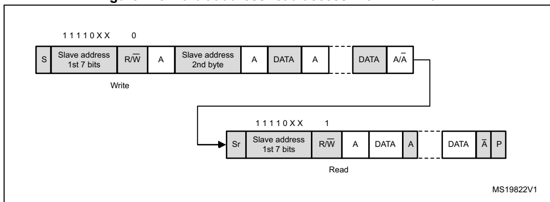
Figure 218. 10-bit address read access with HEAD10R=1
