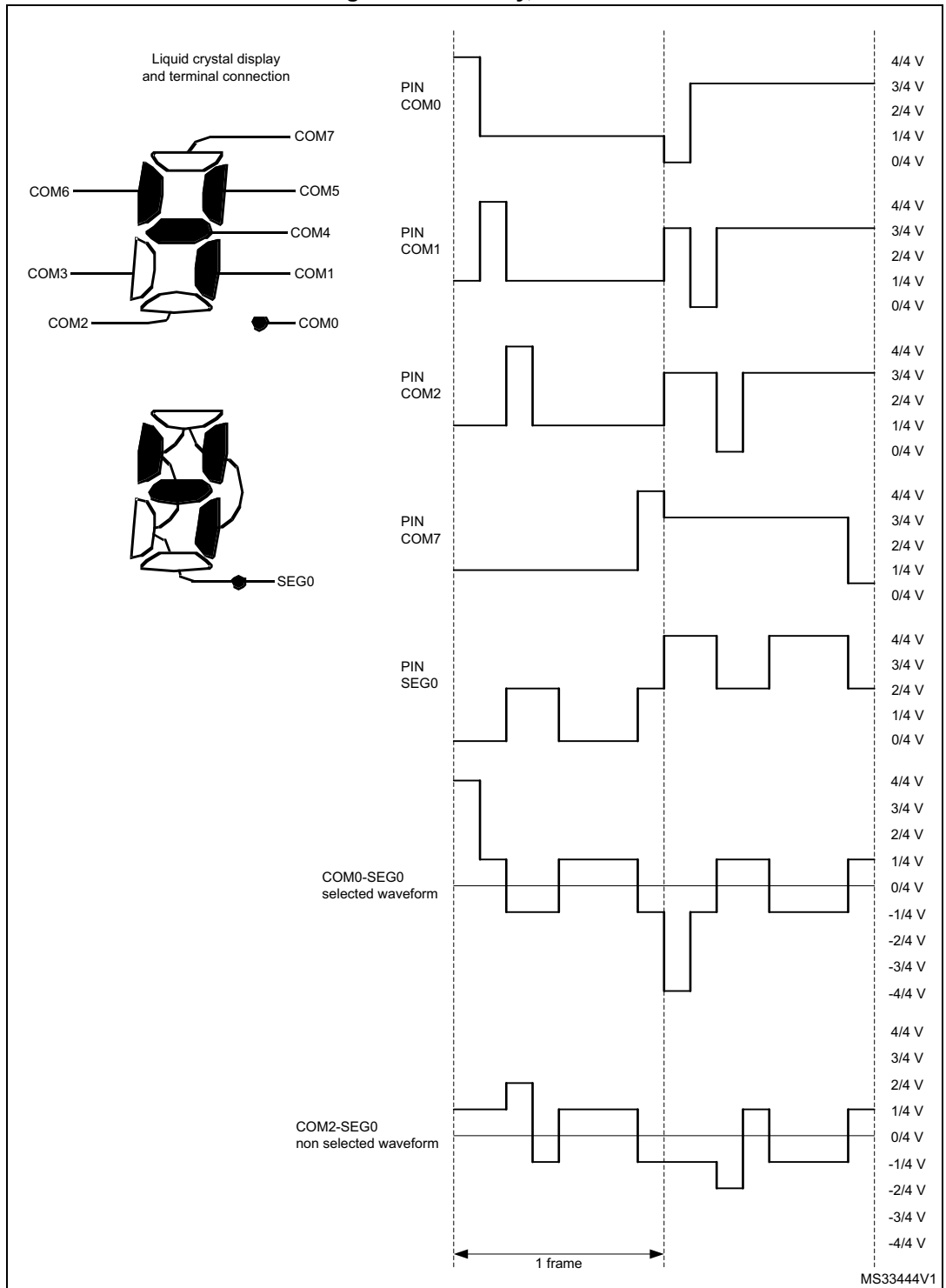
Figure 71. 1/8 duty, 1/4 bias
