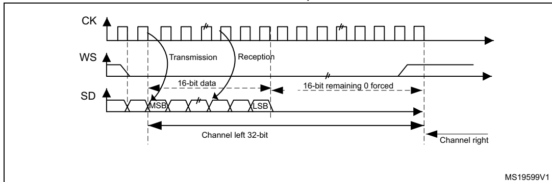
Figure 287. I 2 S Philips standard (16-bit extended to 32-bit packet frame with CPOL = 0)
