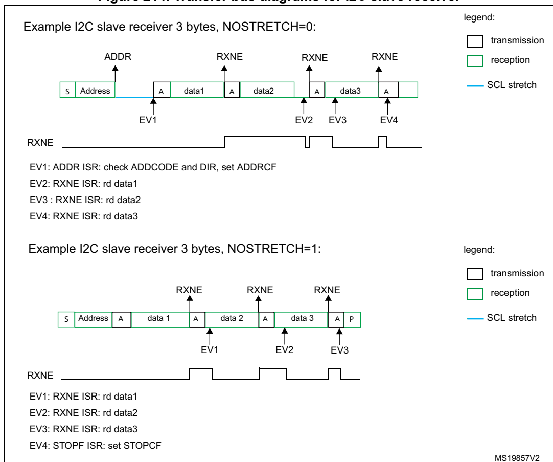
Figure 214. Transfer bus diagrams for I2C slave receiver
