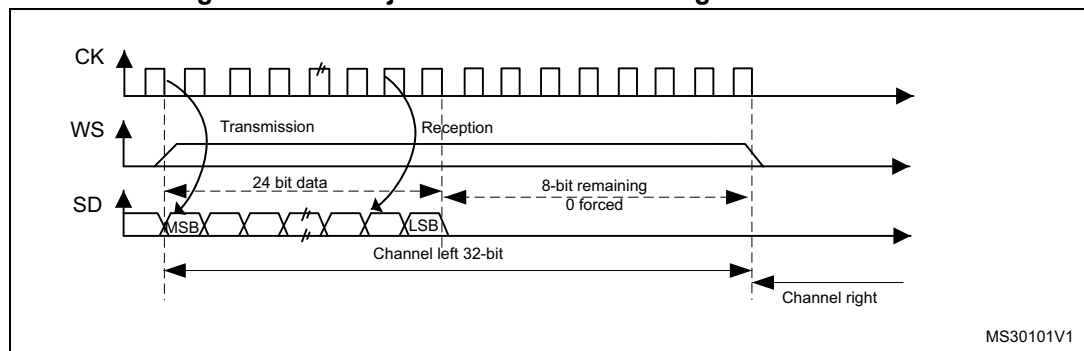
Figure 290. MSB justified 24-bit frame length with CPOL = 0
