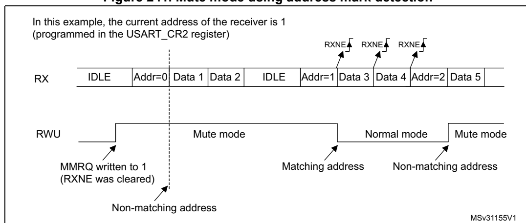
Figure 241. Mute mode using address mark detection
