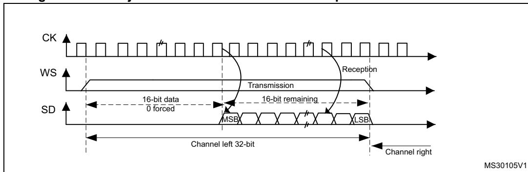
Figure 296. LSB justified 16-bit extended to 32-bit packet frame with CPOL = 0
