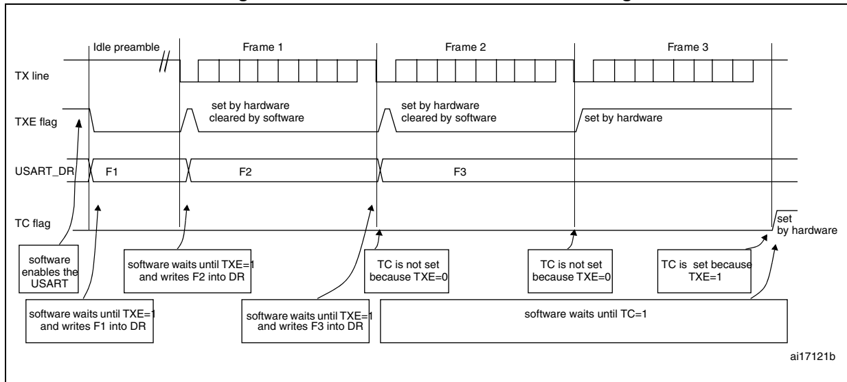
Figure 236. TC/TXE behavior when transmitting
