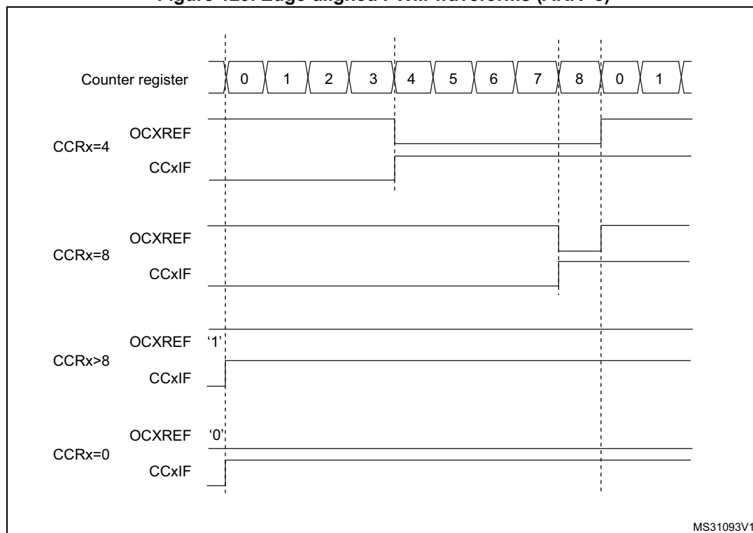
Figure 129. Edge-aligned PWM waveforms (ARR=8)
