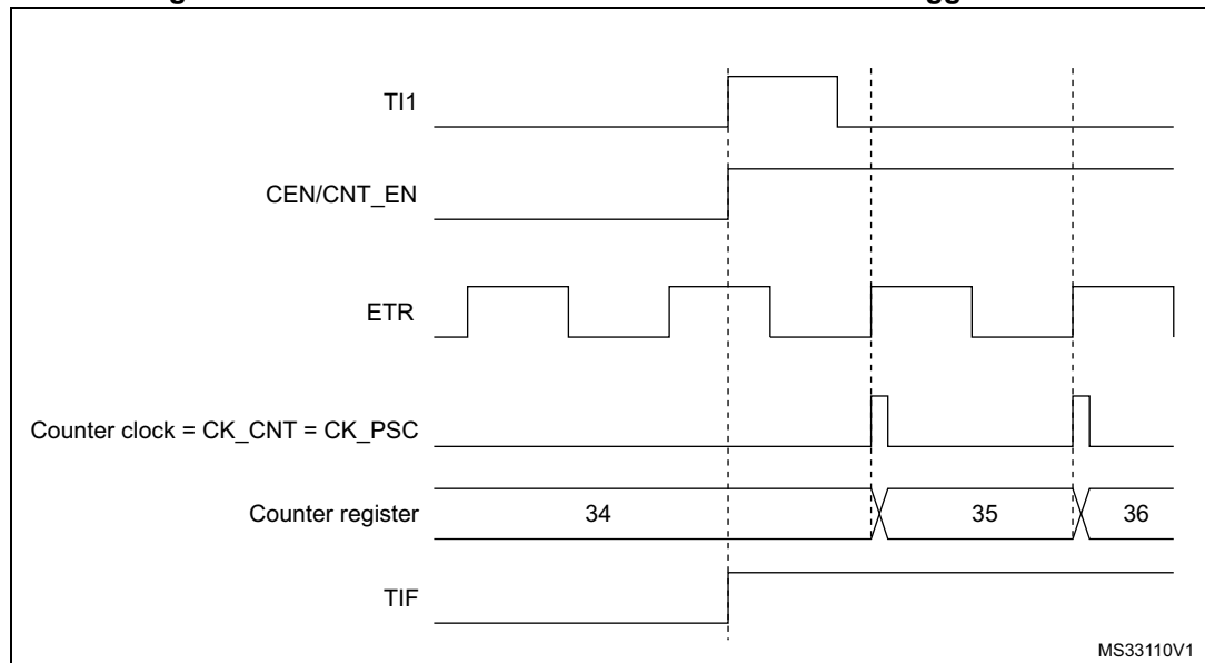
Figure 138. Control circuit in external clock mode 2 + trigger mode
