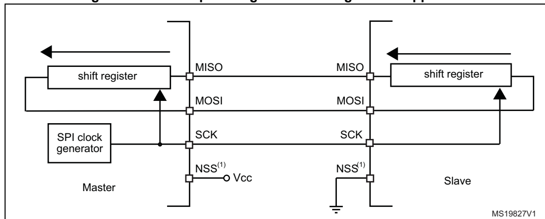
Figure 271. Full-duplex single master/ single slave application
