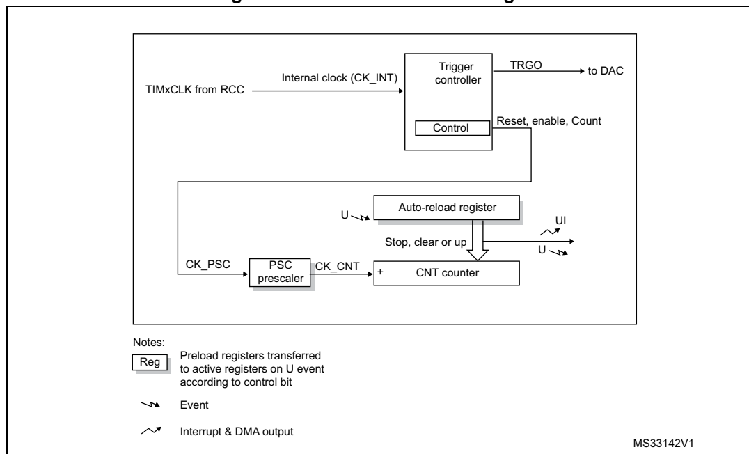
Figure 183. Basic timer block diagram
