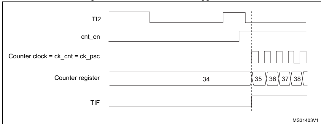
Figure 182. Control circuit in trigger mode
