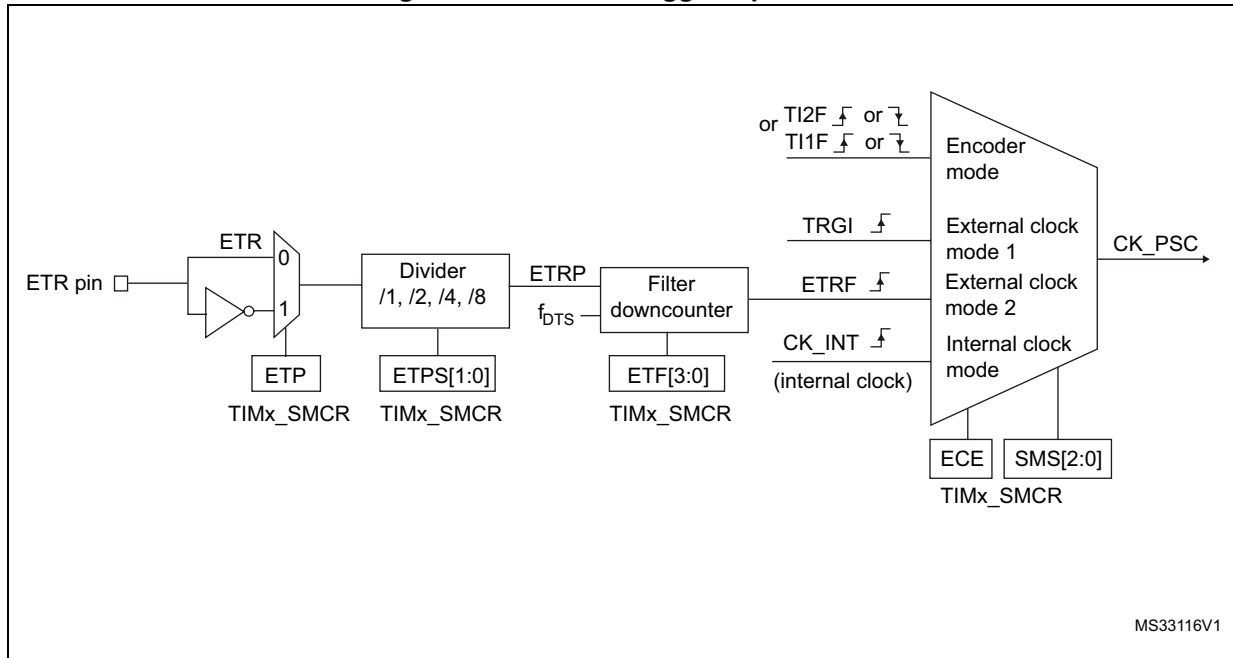
Figure 167. External trigger input block
