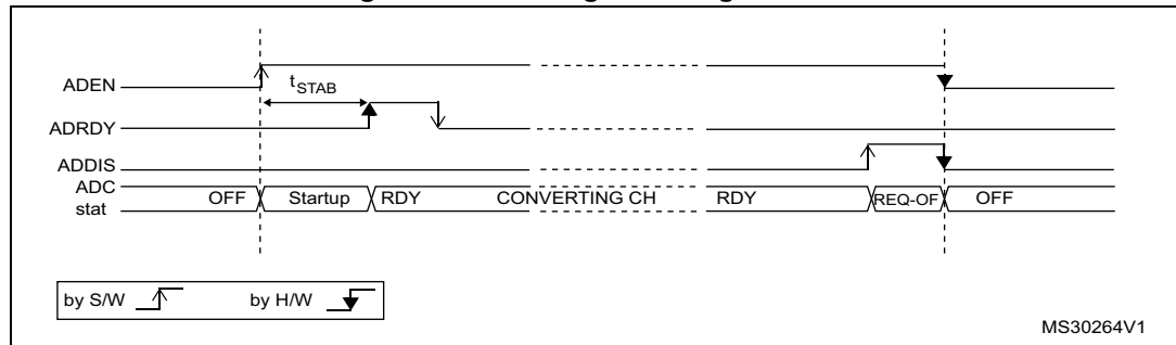
Figure 35. Enabling/disabling the ADC
