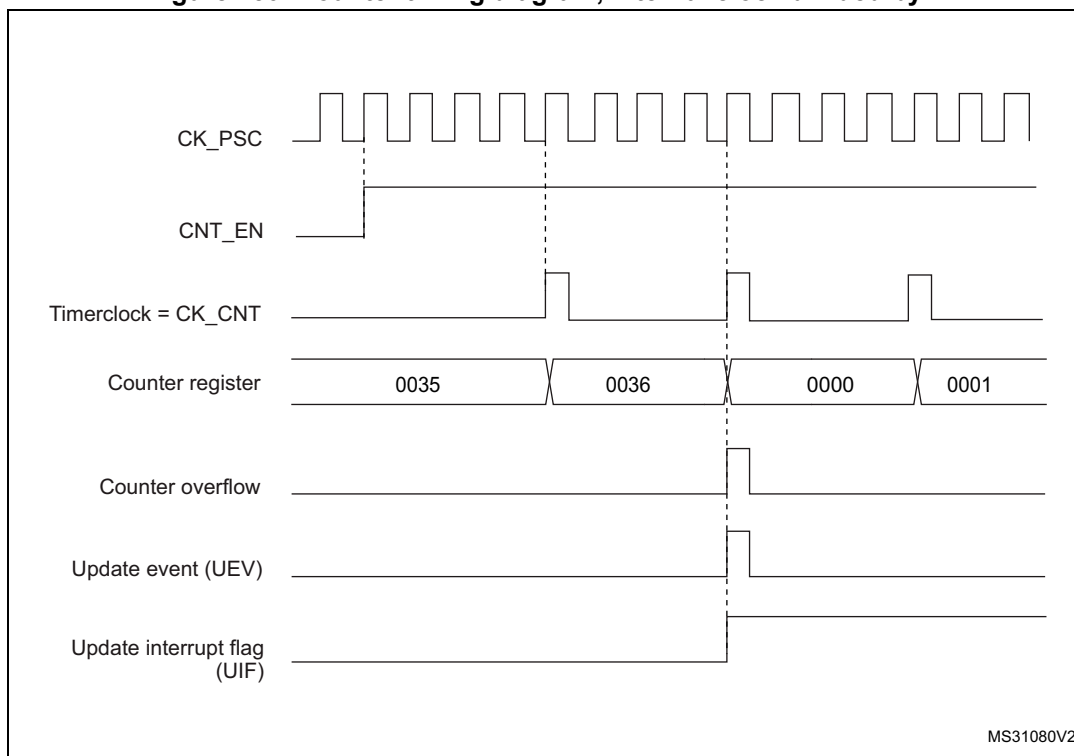
Figure 150. Counter timing diagram, internal clock divided by 4
