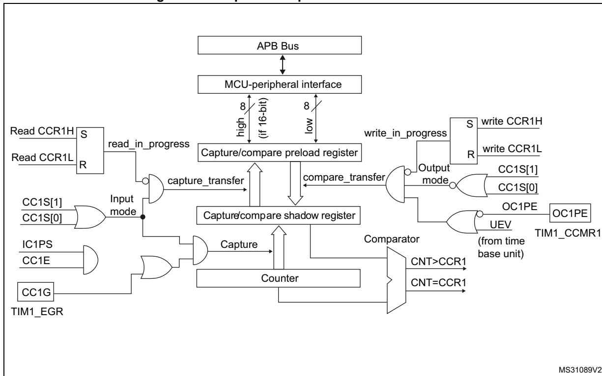
Figure 170. Capture/compare channel 1 main circuit
