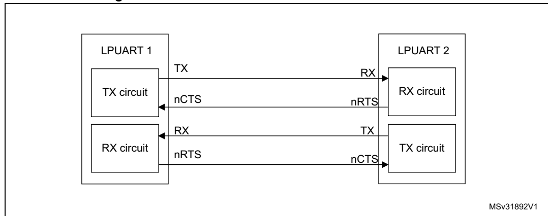
Figure 266. Hardware flow control between 2 LPUARTs
