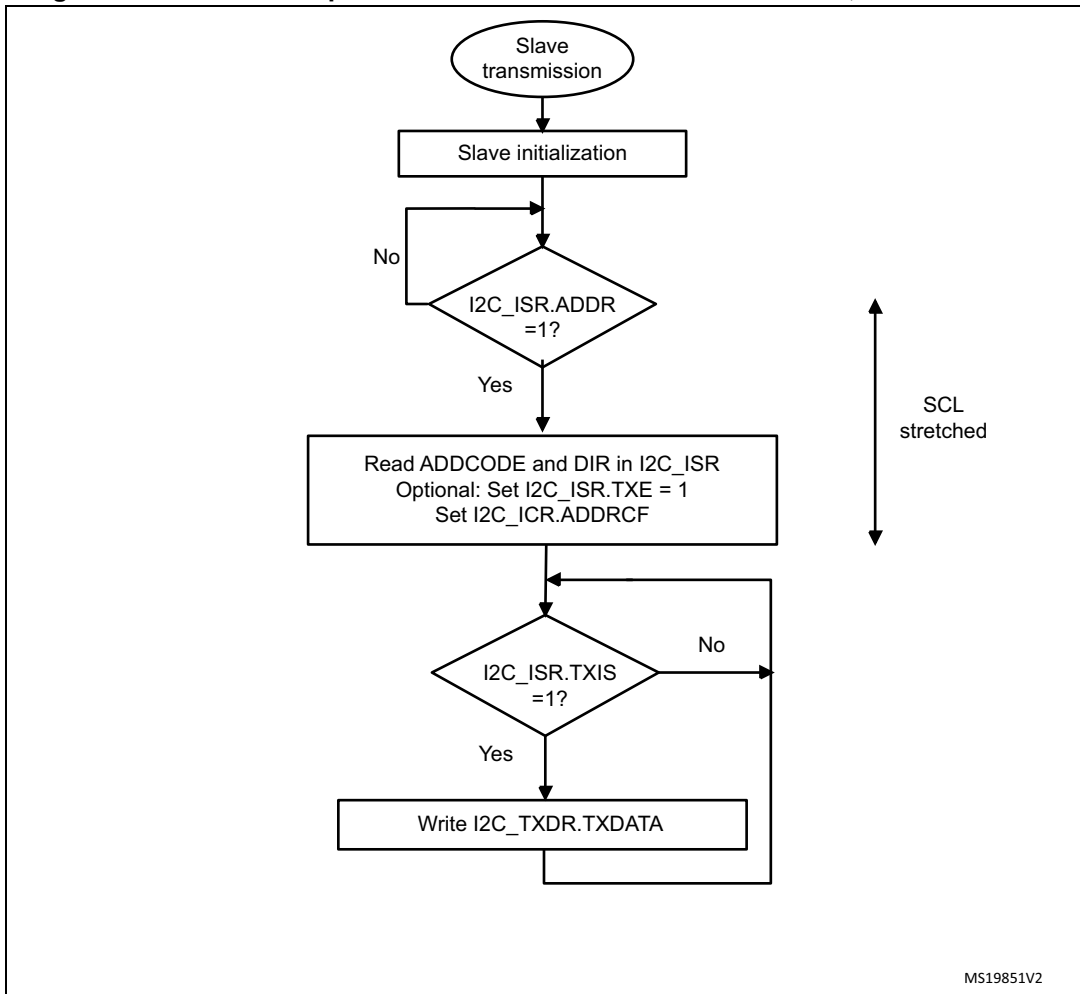
Figure 209. Transfer sequence flowchart for I2C slave transmitter, NOSTRETCH=0
