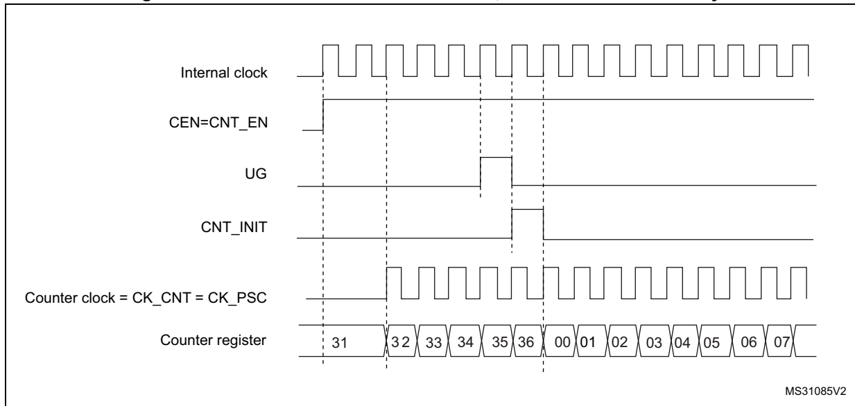
Figure 119. Control circuit in normal mode, internal clock divided by 1
