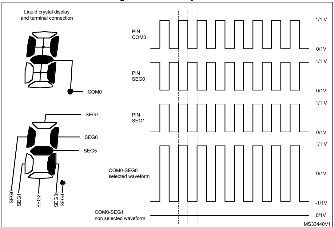
Figure 67. Static duty case 2
