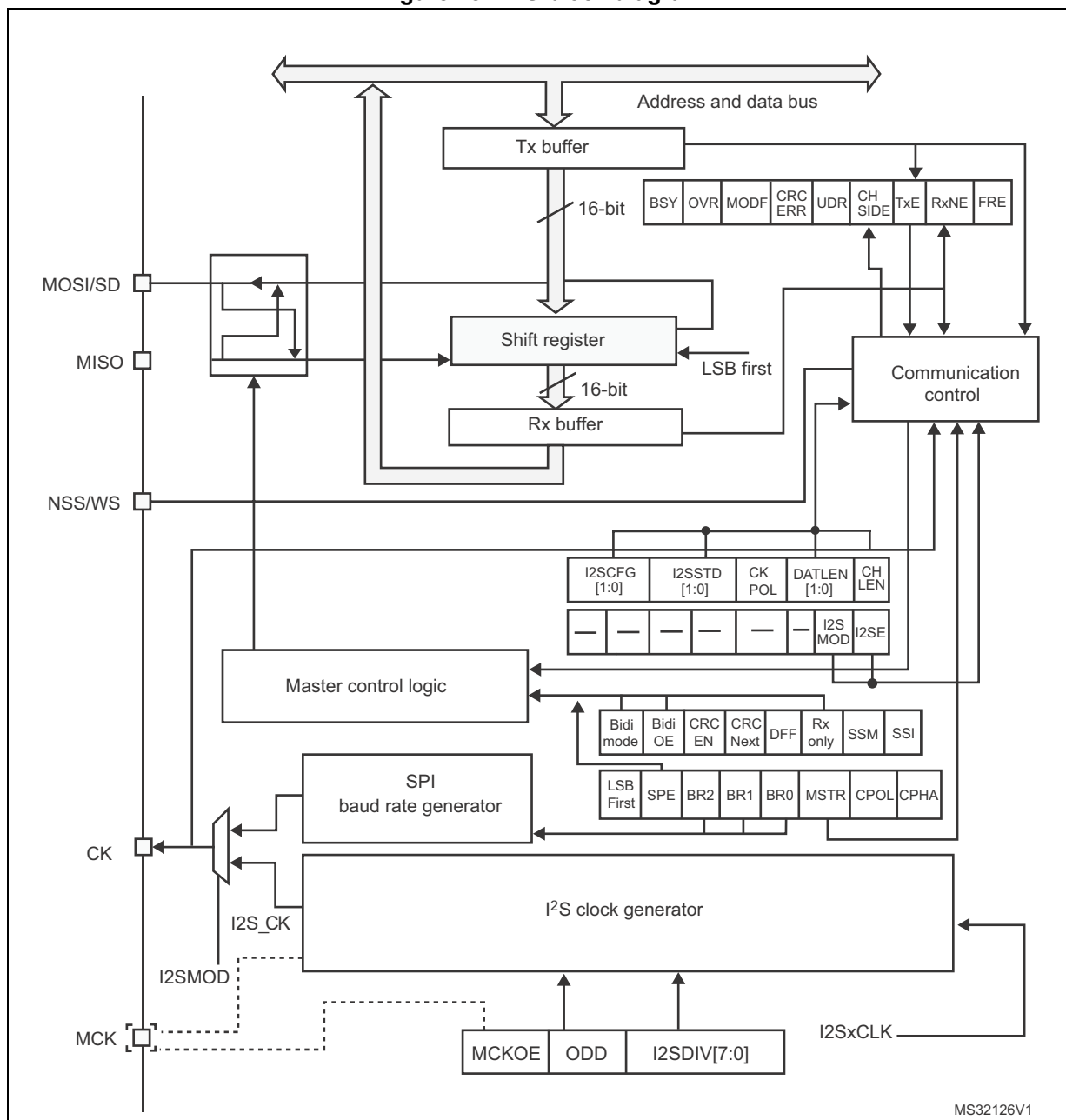
Figure 282. I 2 S block diagram
