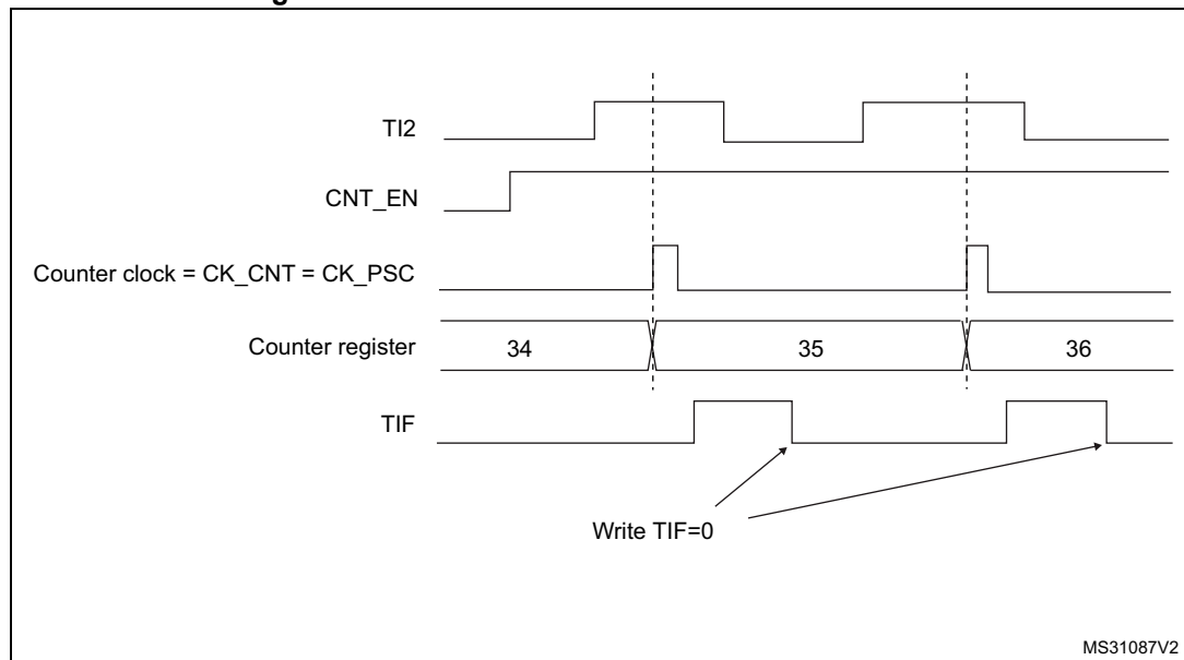
Figure 121. Control circuit in external clock mode 1
