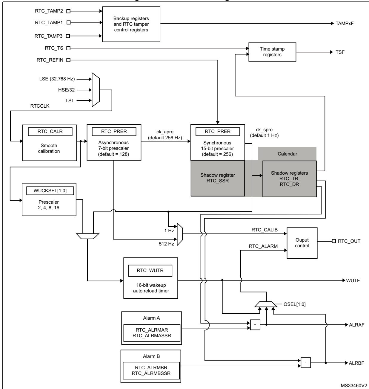
Figure 200. RTC block diagram
