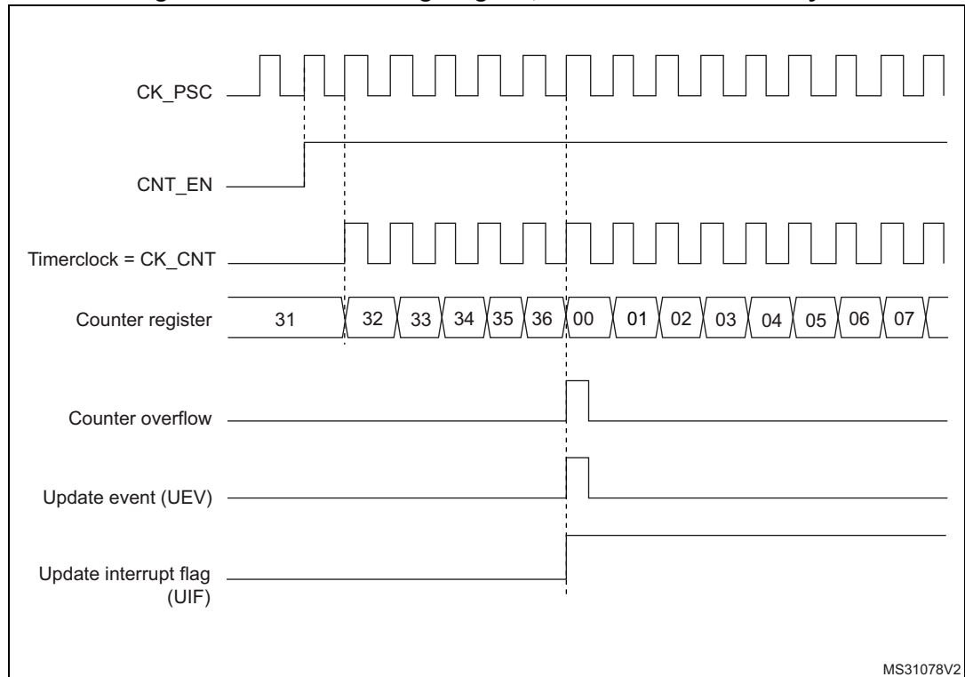
Figure 148. Counter timing diagram, internal clock divided by 1
