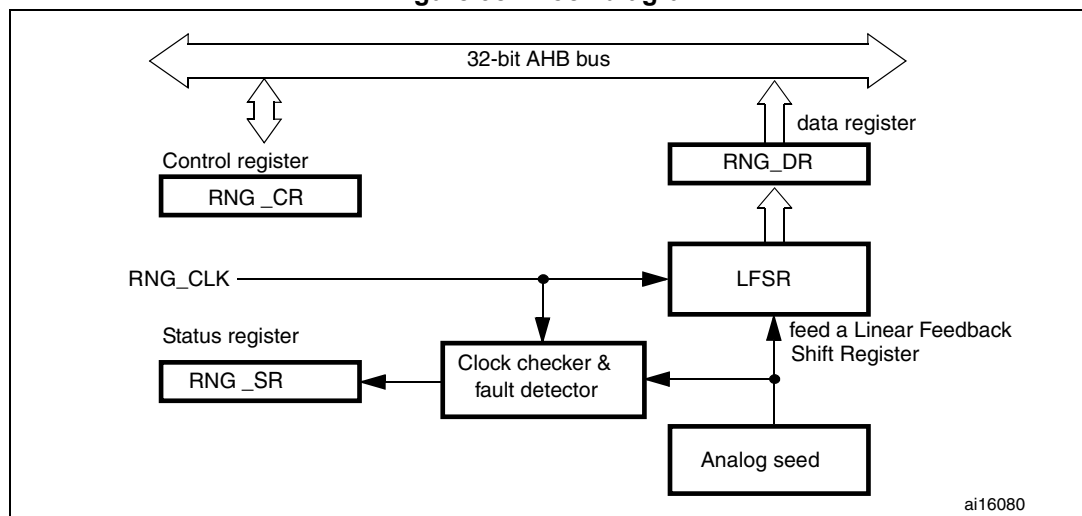
Figure 98. Block diagram
