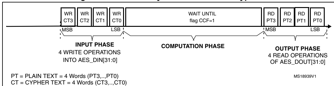
Figure 95. Mode 4: key derivation and decryption
