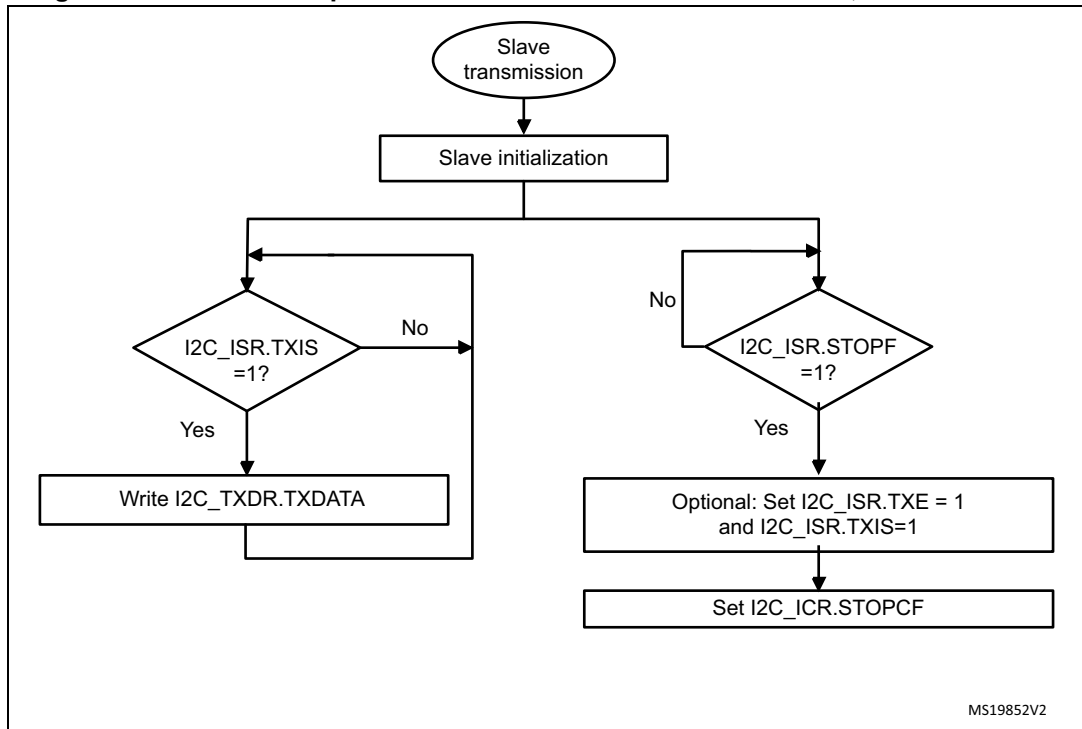
Figure 210. Transfer sequence flowchart for I2C slave transmitter, NOSTRETCH=1
