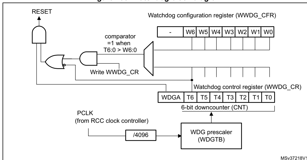
Figure 198. Watchdog block diagram
