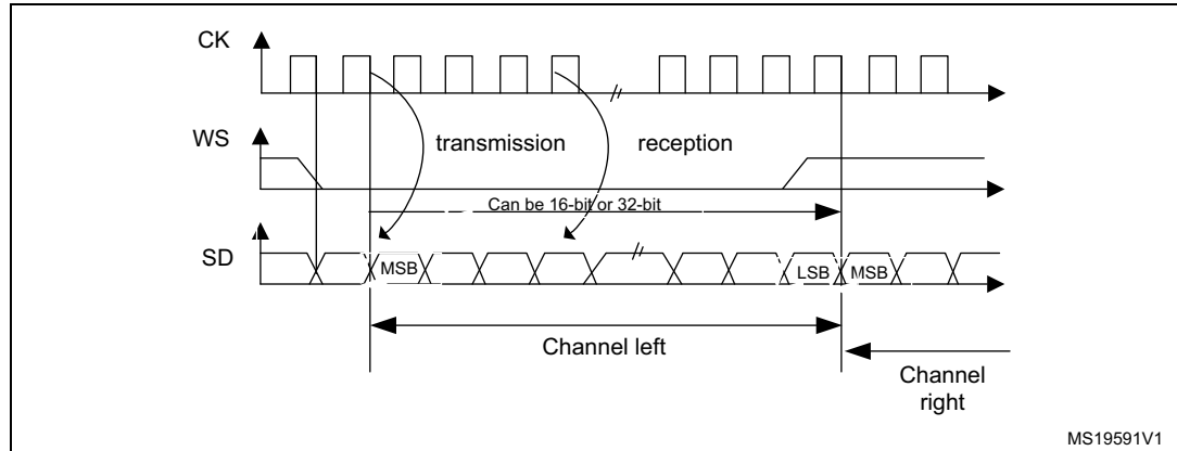
Figure 283. I 2 S Philips protocol waveforms (16/32-bit full accuracy, CPOL = 0)
