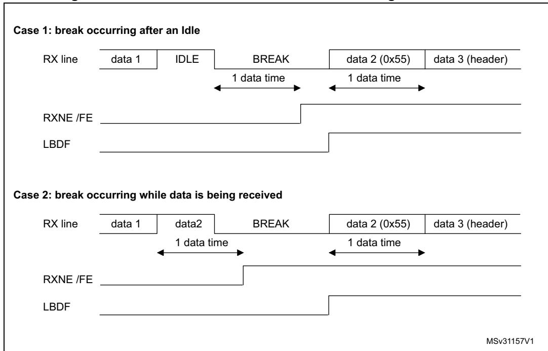
Figure 243. Break detection in LIN mode vs. Framing error detection
