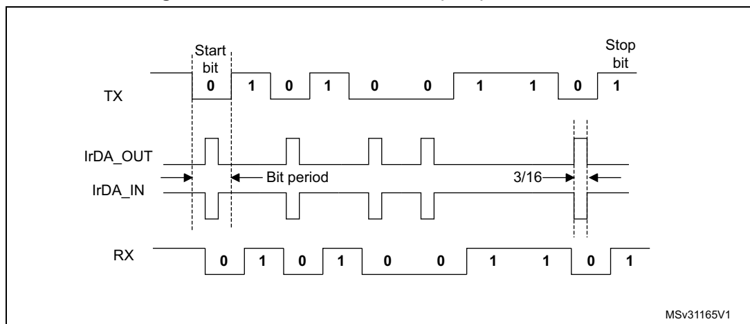
Figure 251. IrDA data modulation (3/16) -Normal Mode
