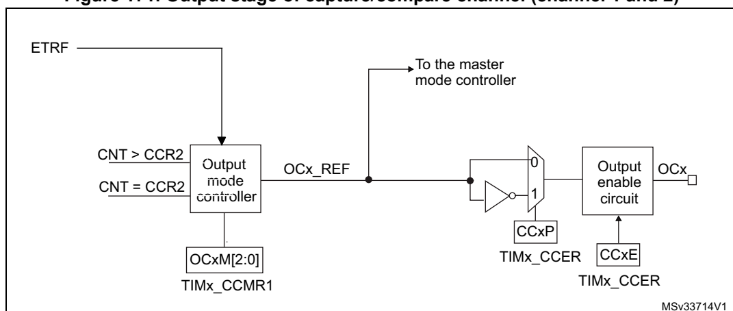
Figure 171. Output stage of capture/compare channel (channel 1 and 2)
