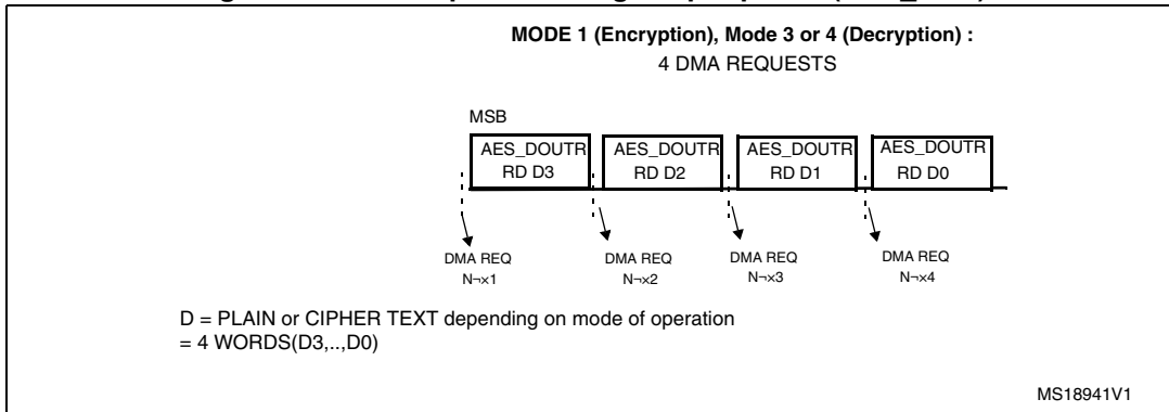
Figure 97. DMA requests during Output phase (AES_OUT)
