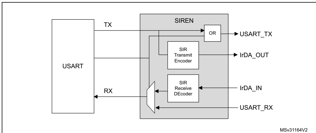
Figure 250. IrDA SIR ENDEC- block diagram
