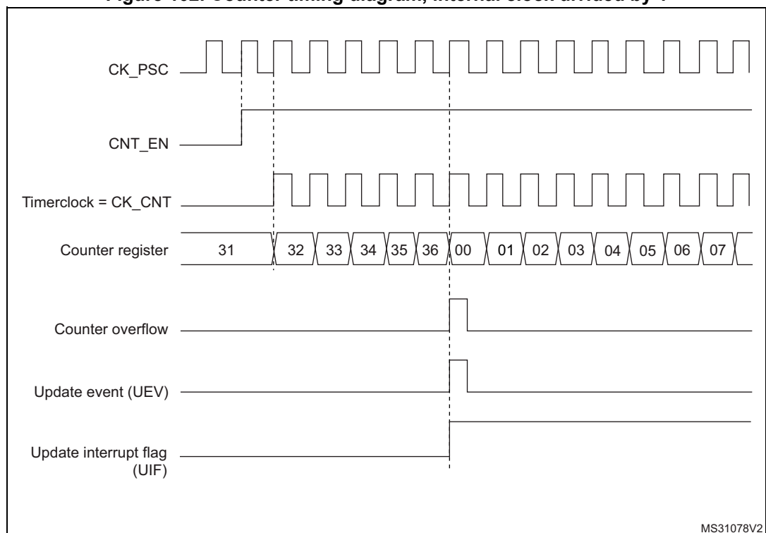
Figure 102. Counter timing diagram, internal clock divided by 1
