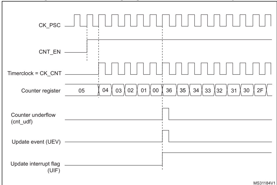
Figure 108. Counter timing diagram, internal clock divided by 1
