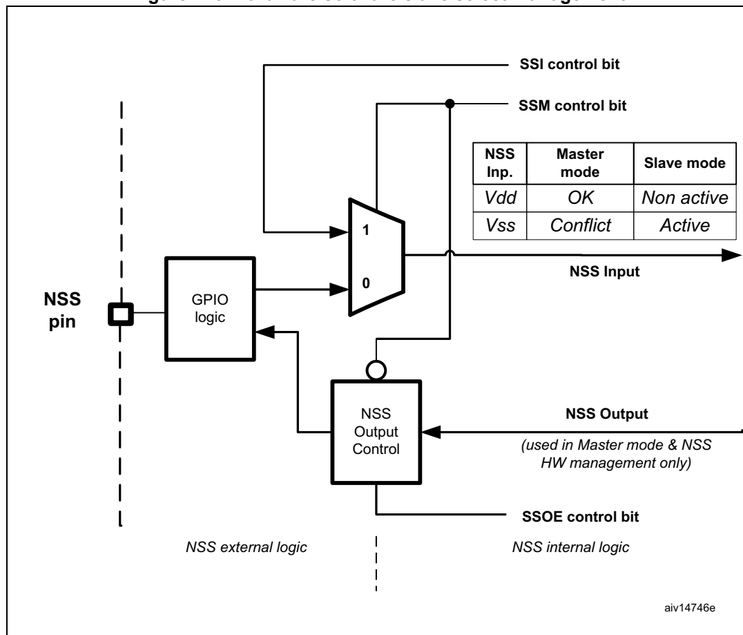
Figure 275. Hardware/software slave select management
