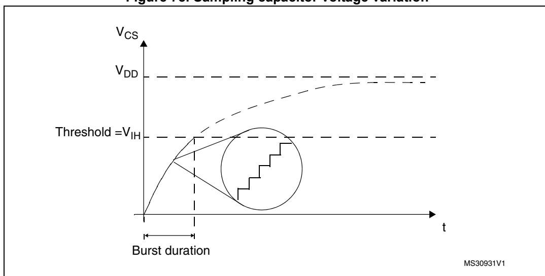
Figure 78. Sampling capacitor voltage variation
