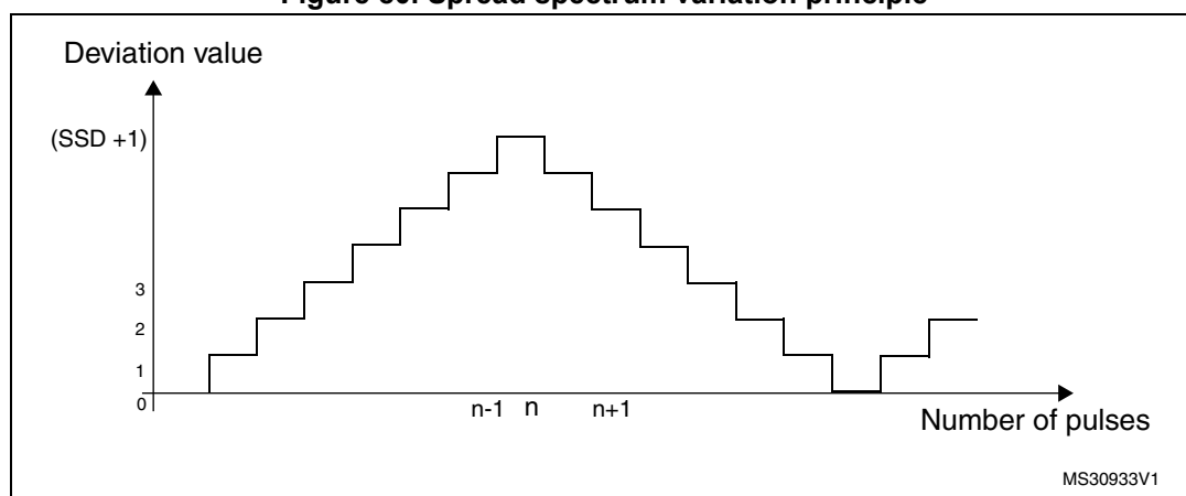
Figure 80. Spread spectrum variation principle
