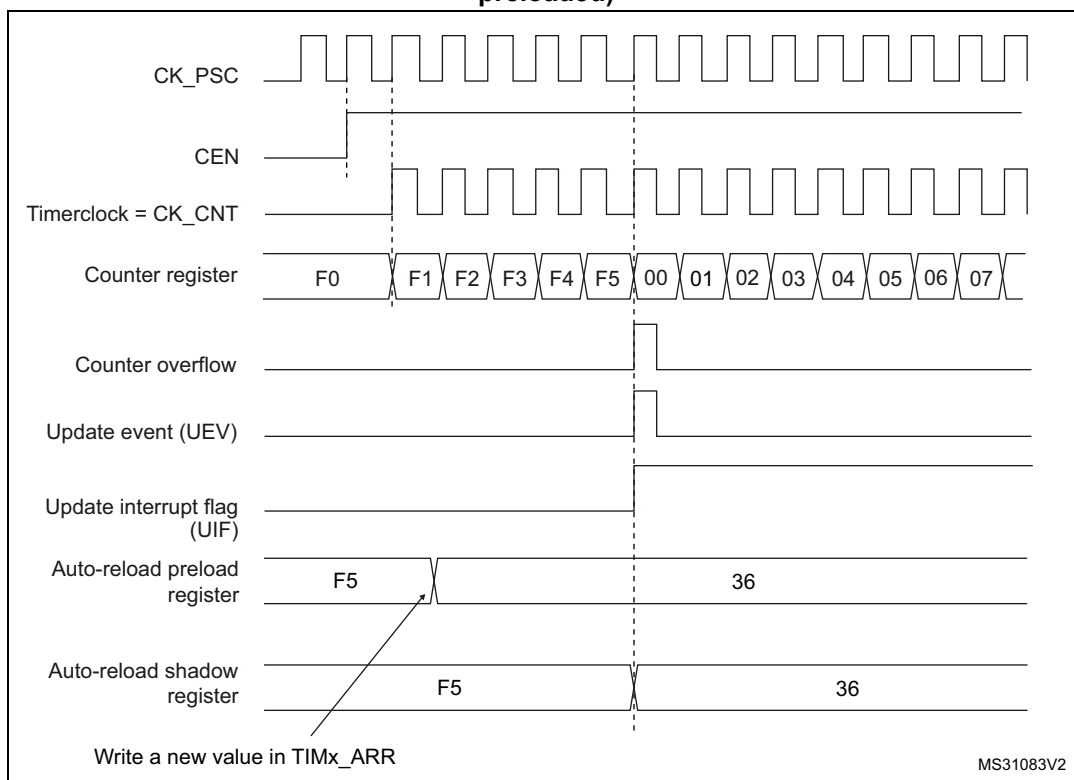
Figure 153. Counter timing diagram, update event when ARPE=1 (TIMx_ARR preloaded)
