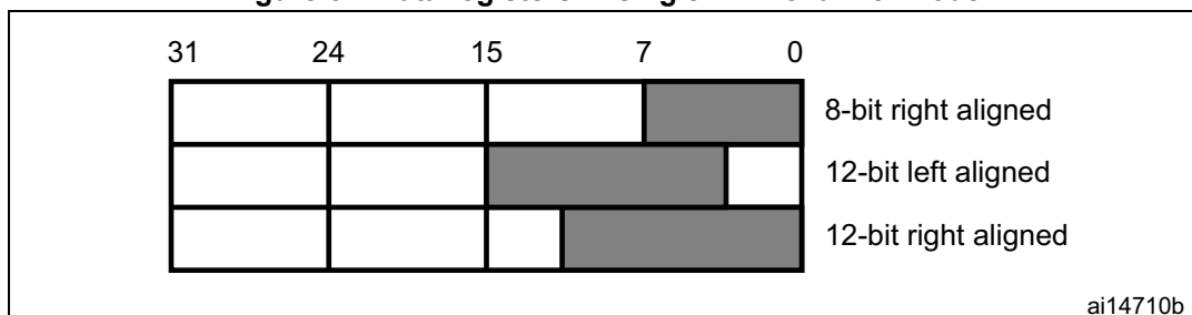
Figure 57. Data registers in single DAC channel mode
