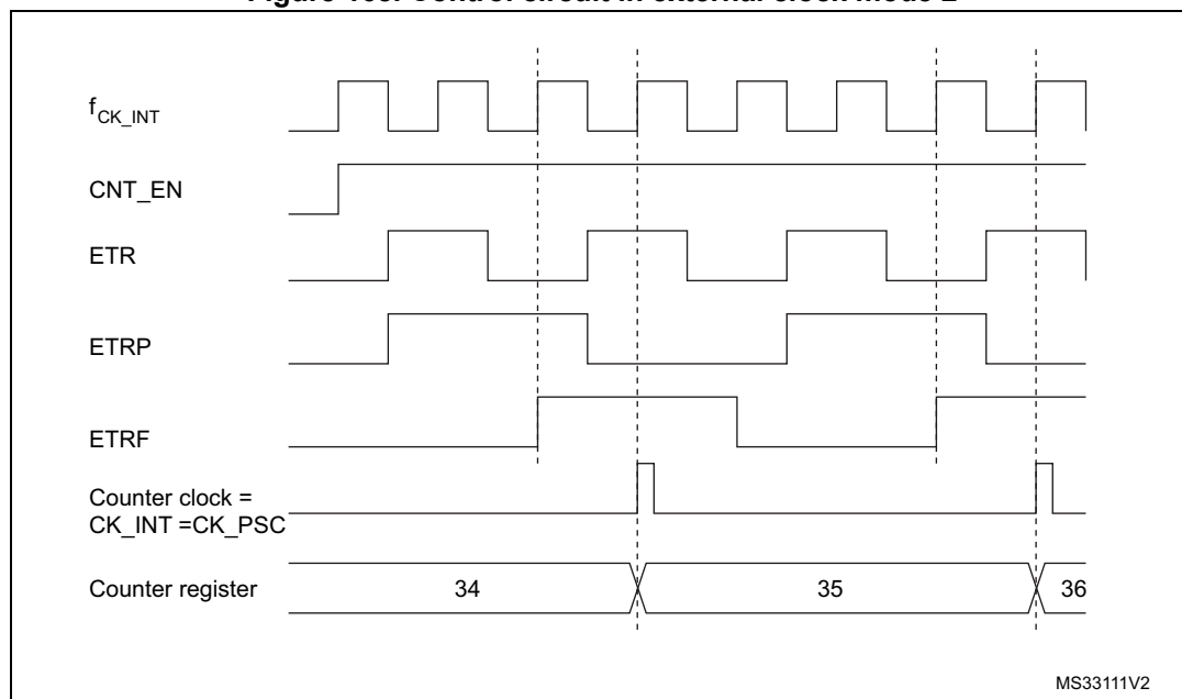
Figure 168. Control circuit in external clock mode 2
