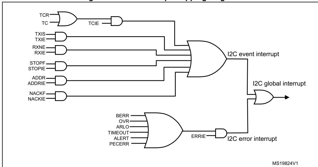
Figure 232. I2C interrupt mapping diagram
