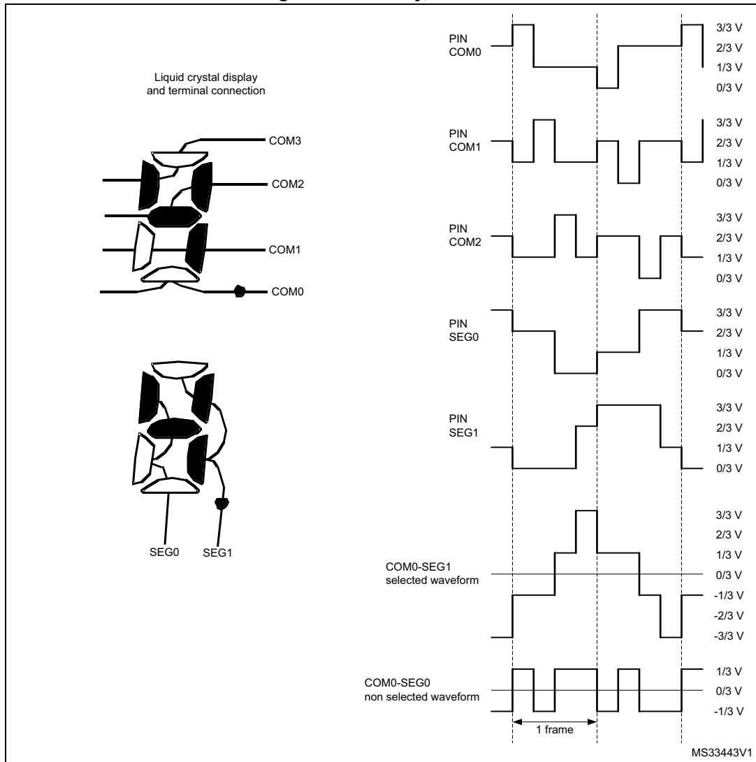
Figure 70. 1/4 duty, 1/3 bias
