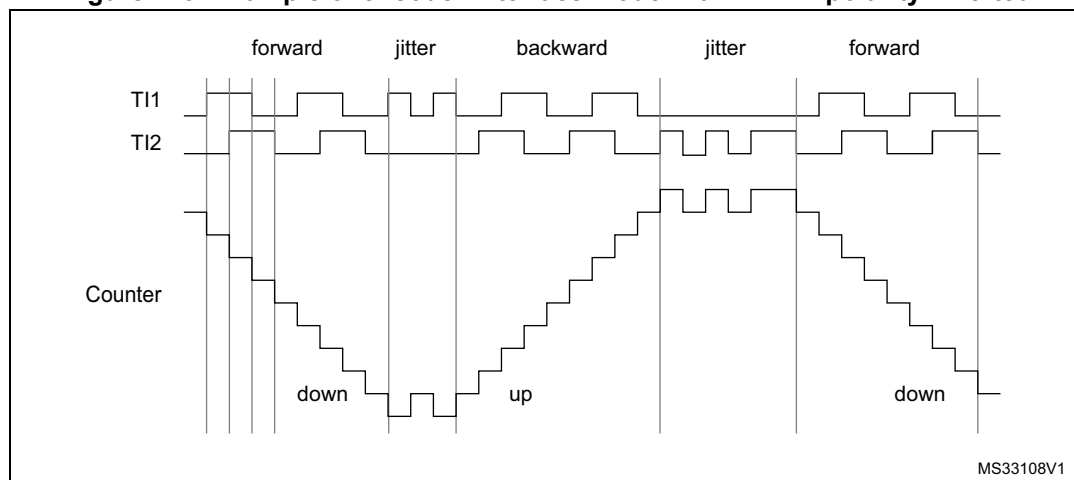
Figure 179. Example of encoder interface mode with TI1FP1 polarity inverted
