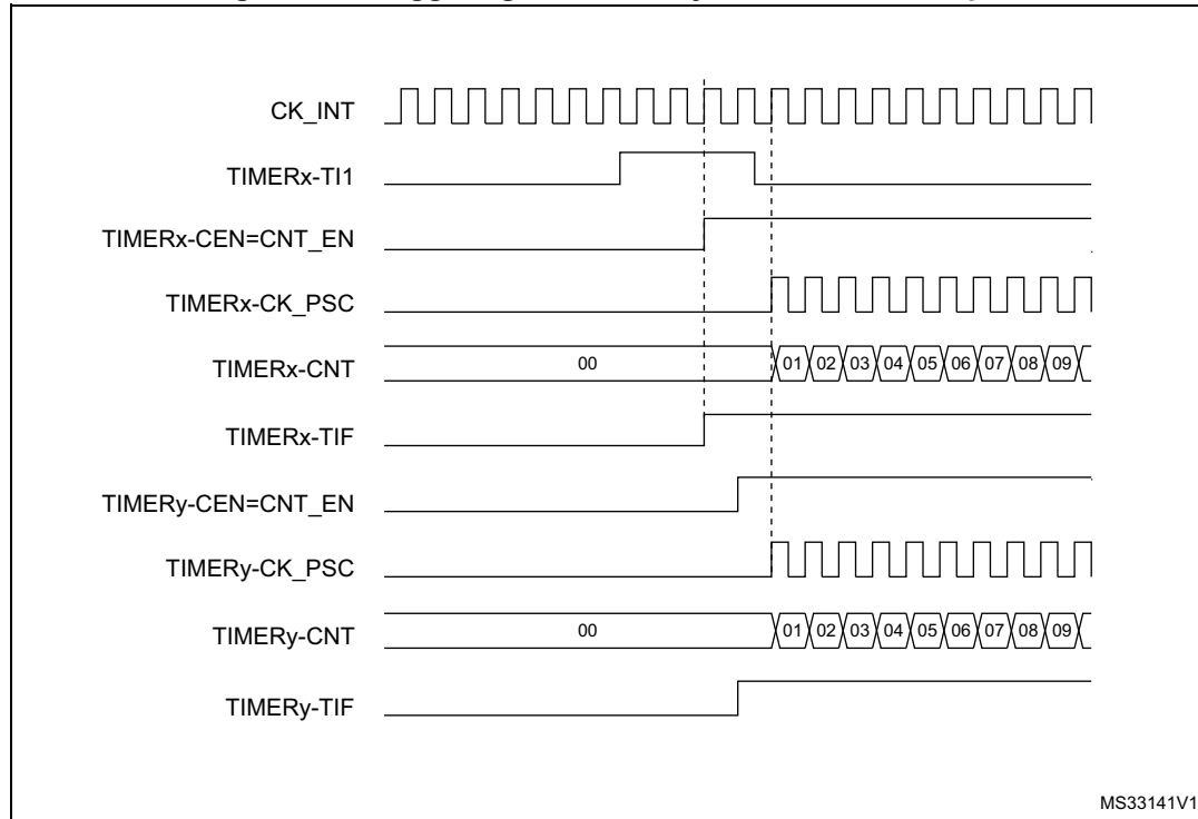
Figure 144. Triggering timer x and y with timer x TI1 input
