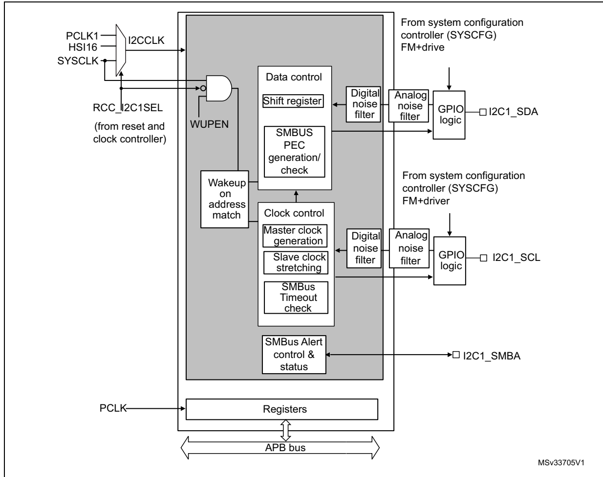
Figure 201. I2C1/3 block diagram
