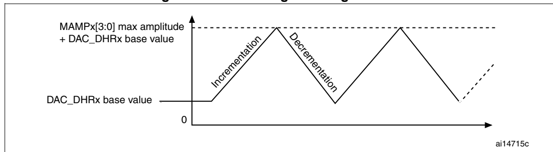
Figure 62. DAC conversion (SW trigger enabled) with triangle wave generation
