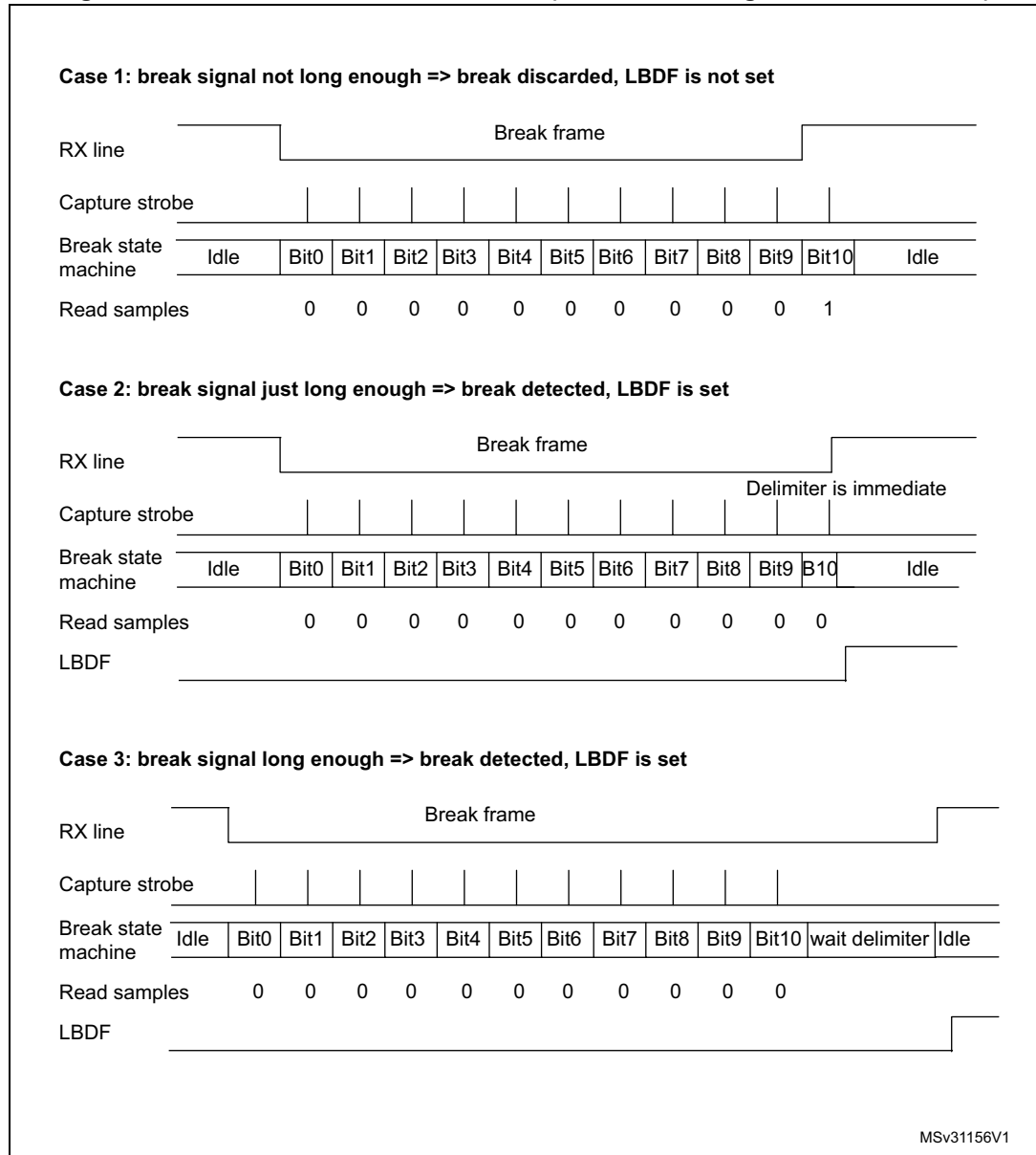
Figure 242. Break detection in LIN mode (11-bit break length - LBDL bit is set)
