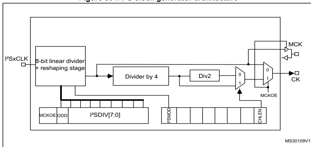
Figure 301. I 2 S clock generator architecture
