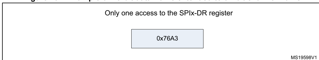
Figure 297. Example of 16-bit data frame extended to 32-bit channel frame
