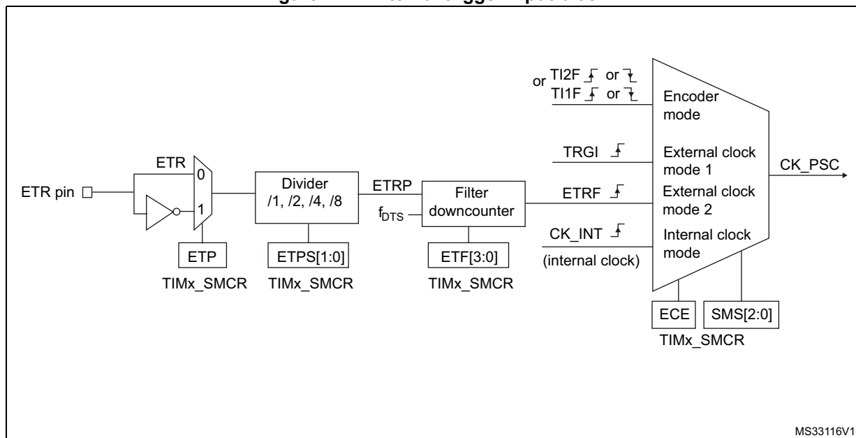
Figure 122. External trigger input block
