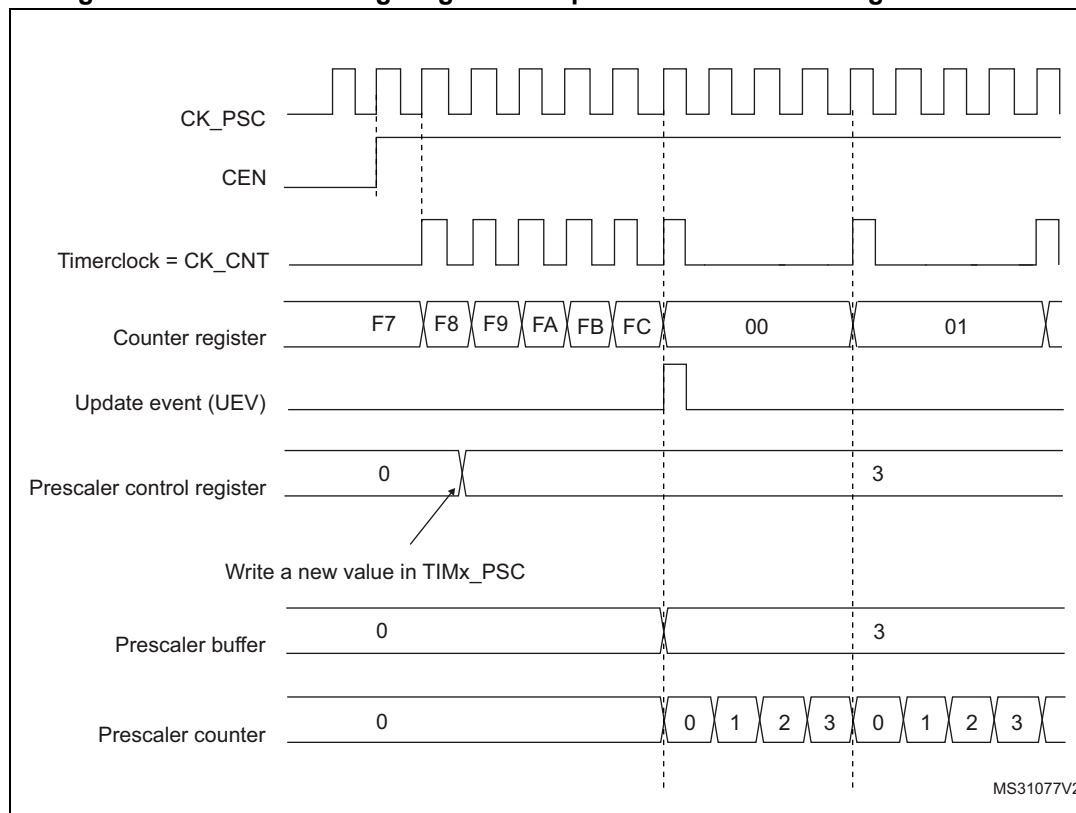
Figure 101. Counter timing diagram with prescaler division change from 1 to 4
