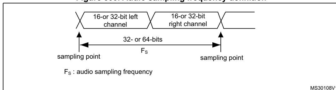
Figure 300. Audio sampling frequency definition
