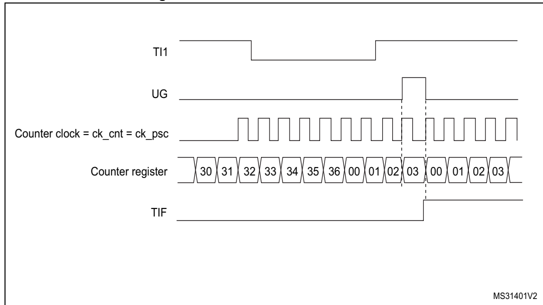
Figure 180. Control circuit in reset mode
