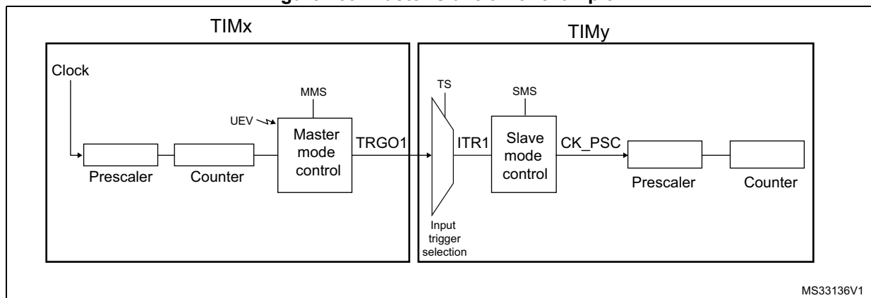
Figure 139. Master/Slave timer example
