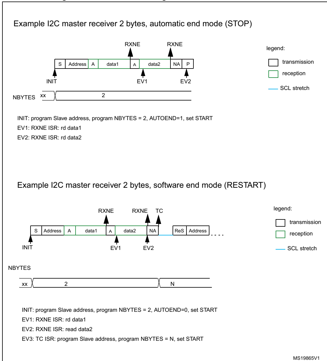
Figure 224. Transfer bus diagrams for I2C master receiver
