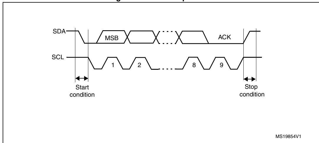
Figure 203. I 2 C bus protocol
