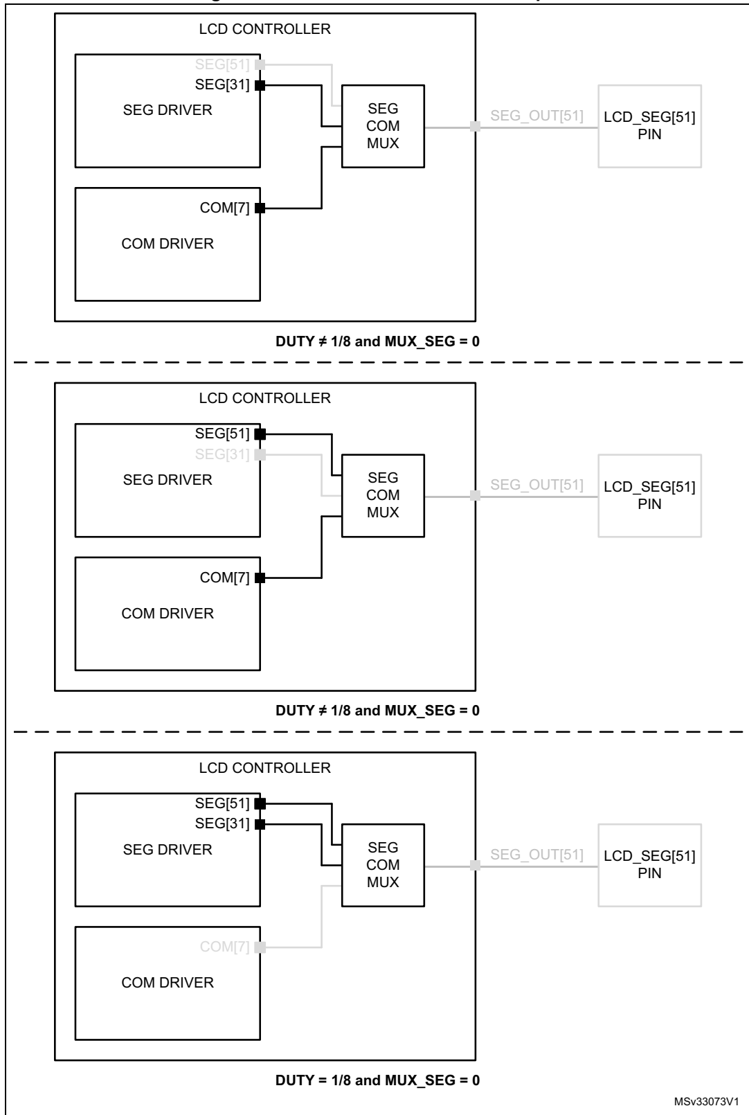
Figure 74. SEG/COM mux feature example
