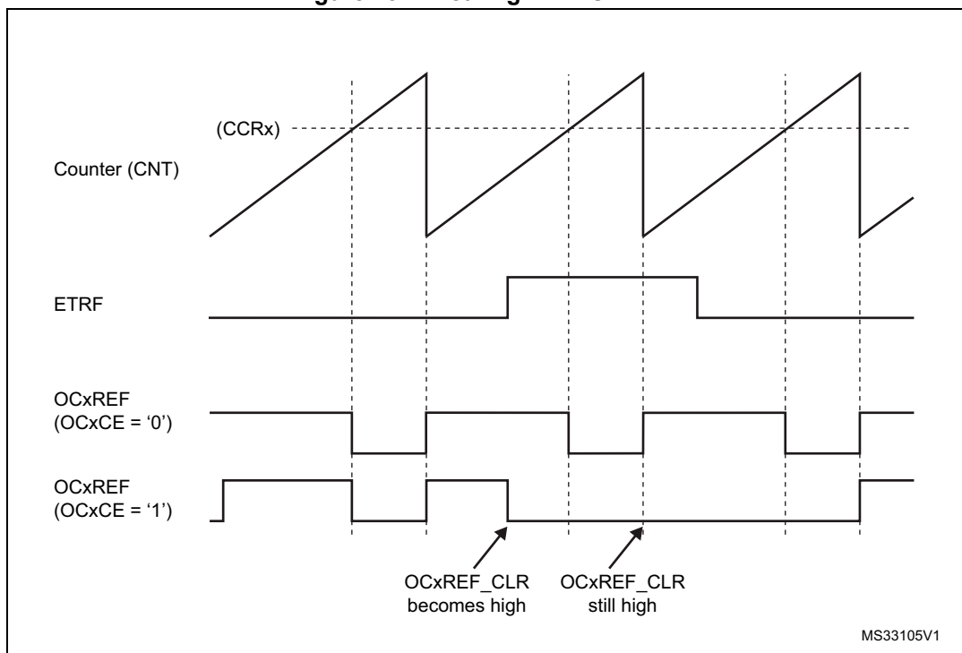
Figure 132. Clearing TIMx OCxREF
