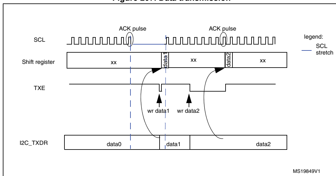
Figure 207. Data transmission
