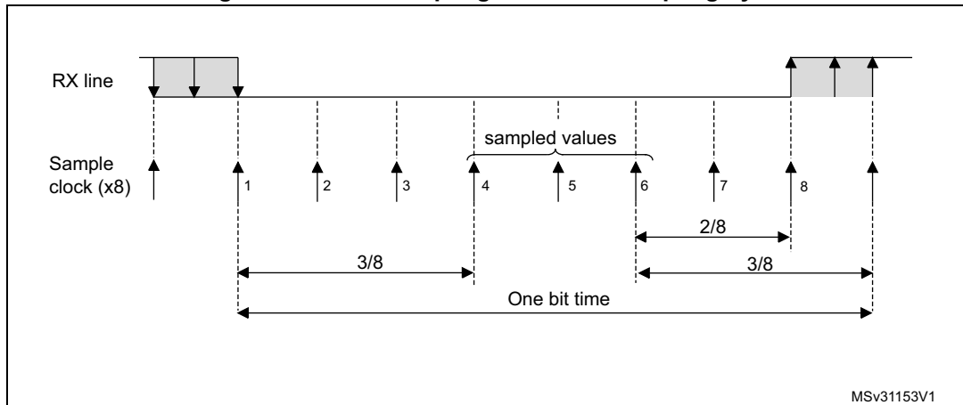
Figure 239. Data sampling when oversampling by 8
