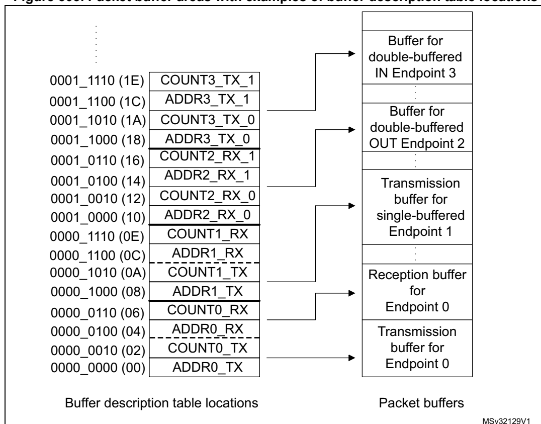
Figure 303. Packet buffer areas with examples of buffer description table locations
