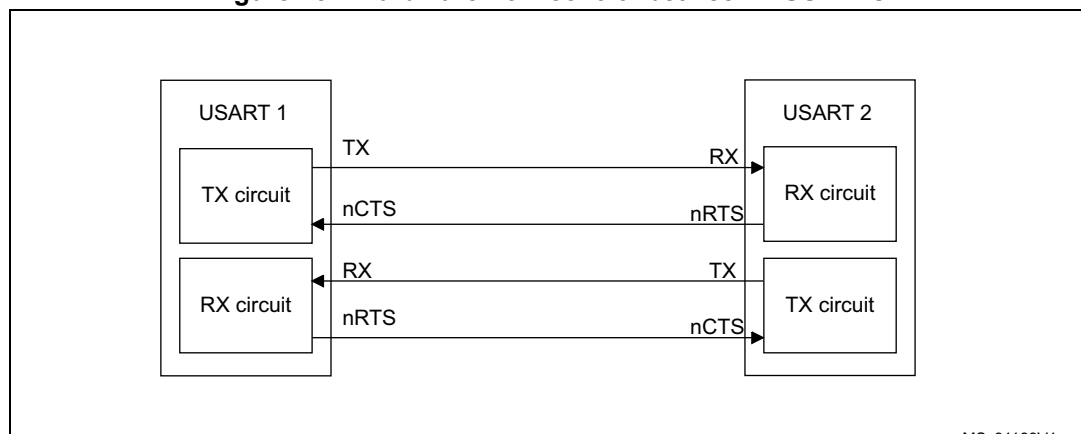
Figure 254. Hardware flow control between 2 USARTs
