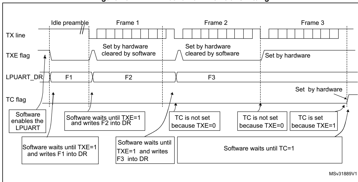
Figure 261. TC/TXE behavior when transmitting
