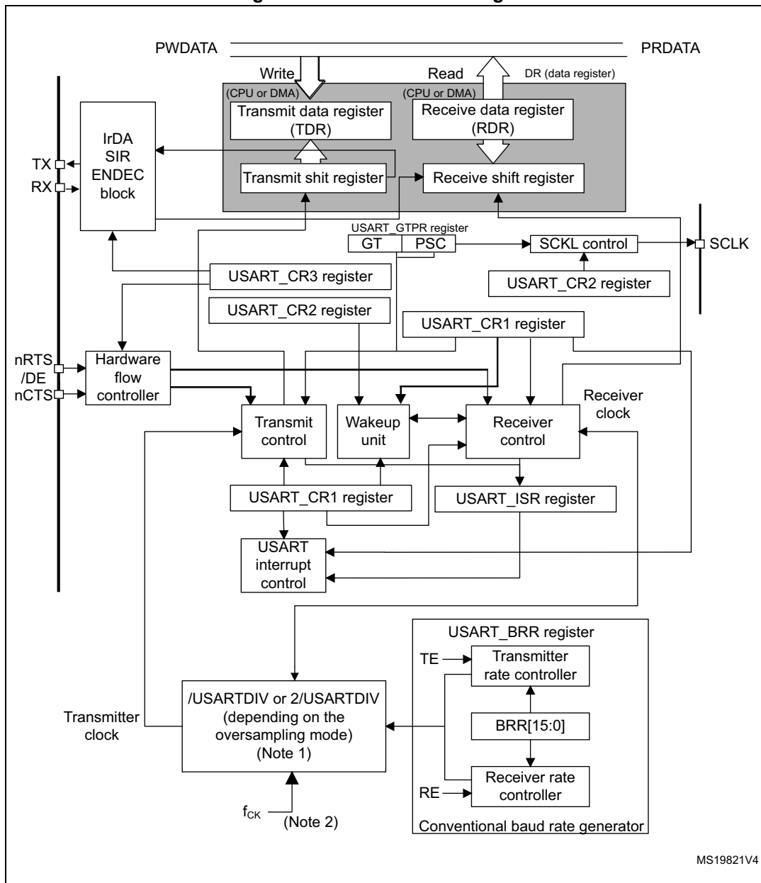
Figure 233. USART block diagram
