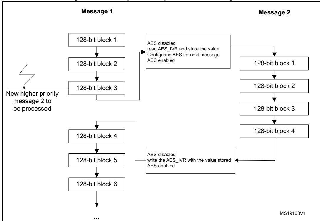
Figure 86. Example of suspend mode management
