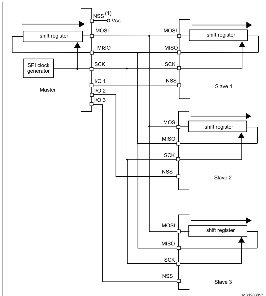
Figure 274. Master and three independent slaves
