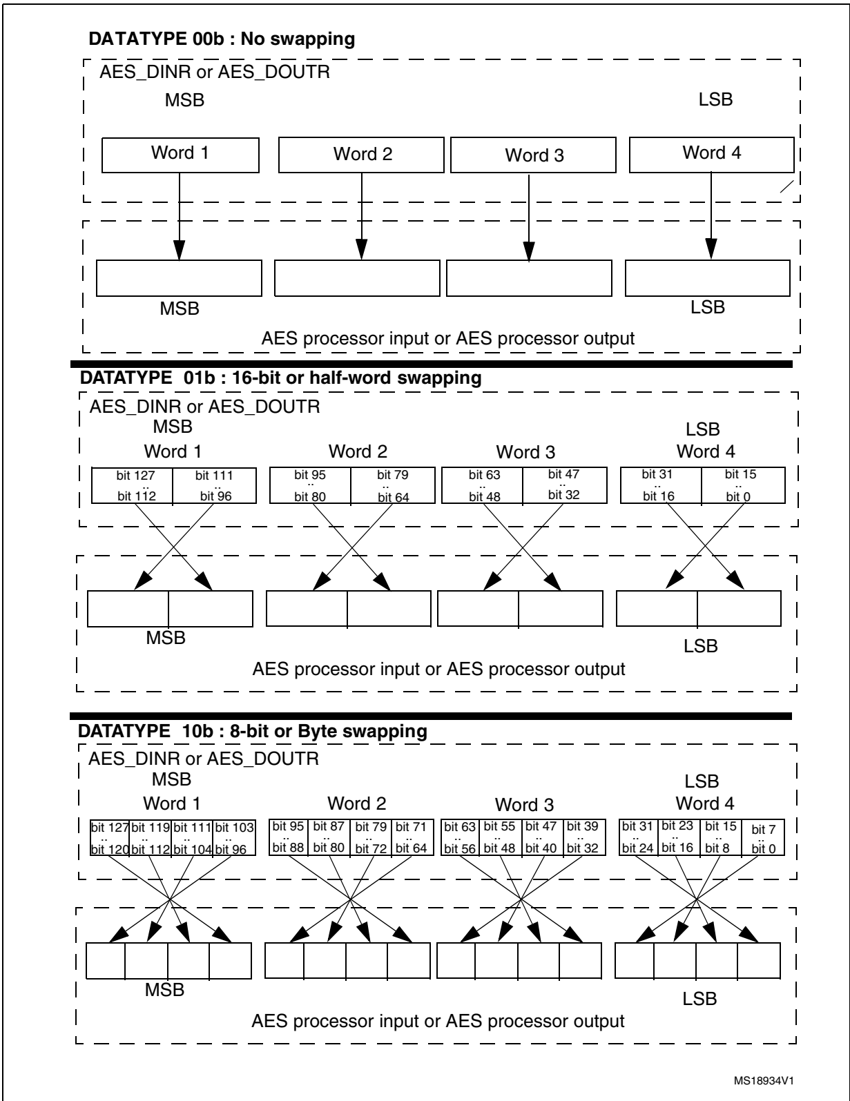
Figure 90. 128-bit block construction according to the data type
