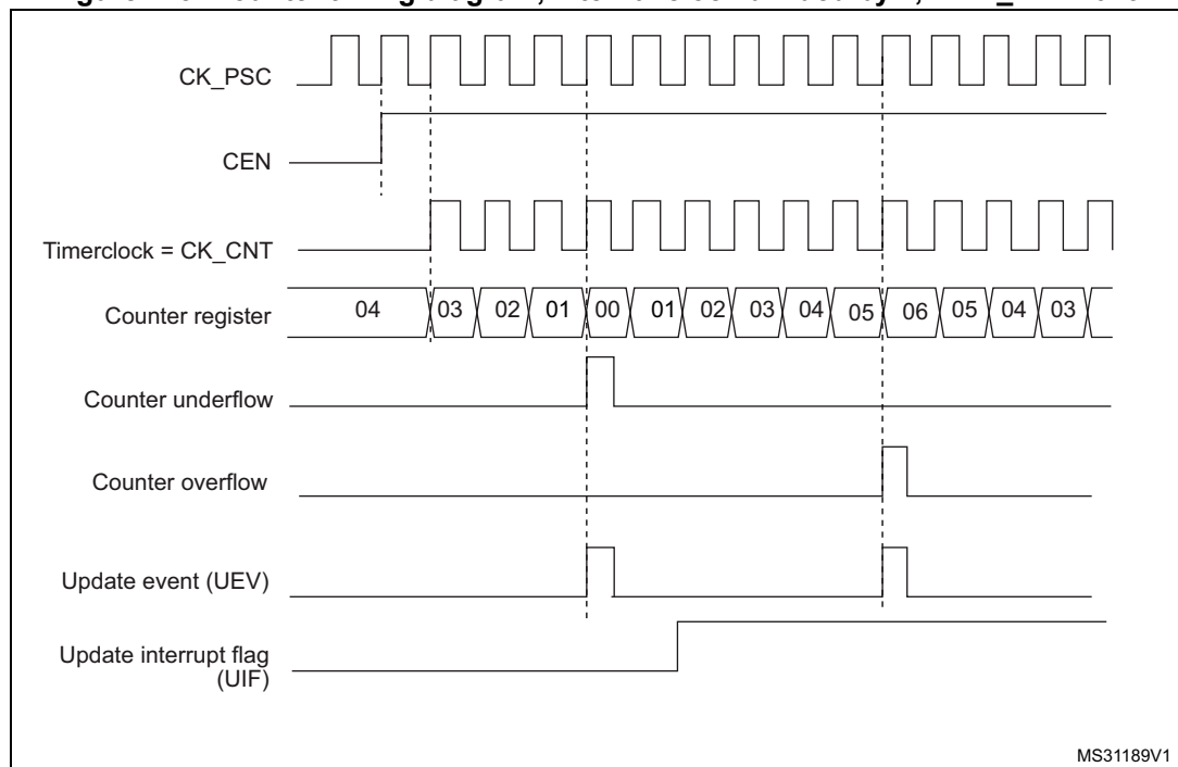
Figure 113. Counter timing diagram, internal clock divided by 1, TIMx_ARR=0x6
