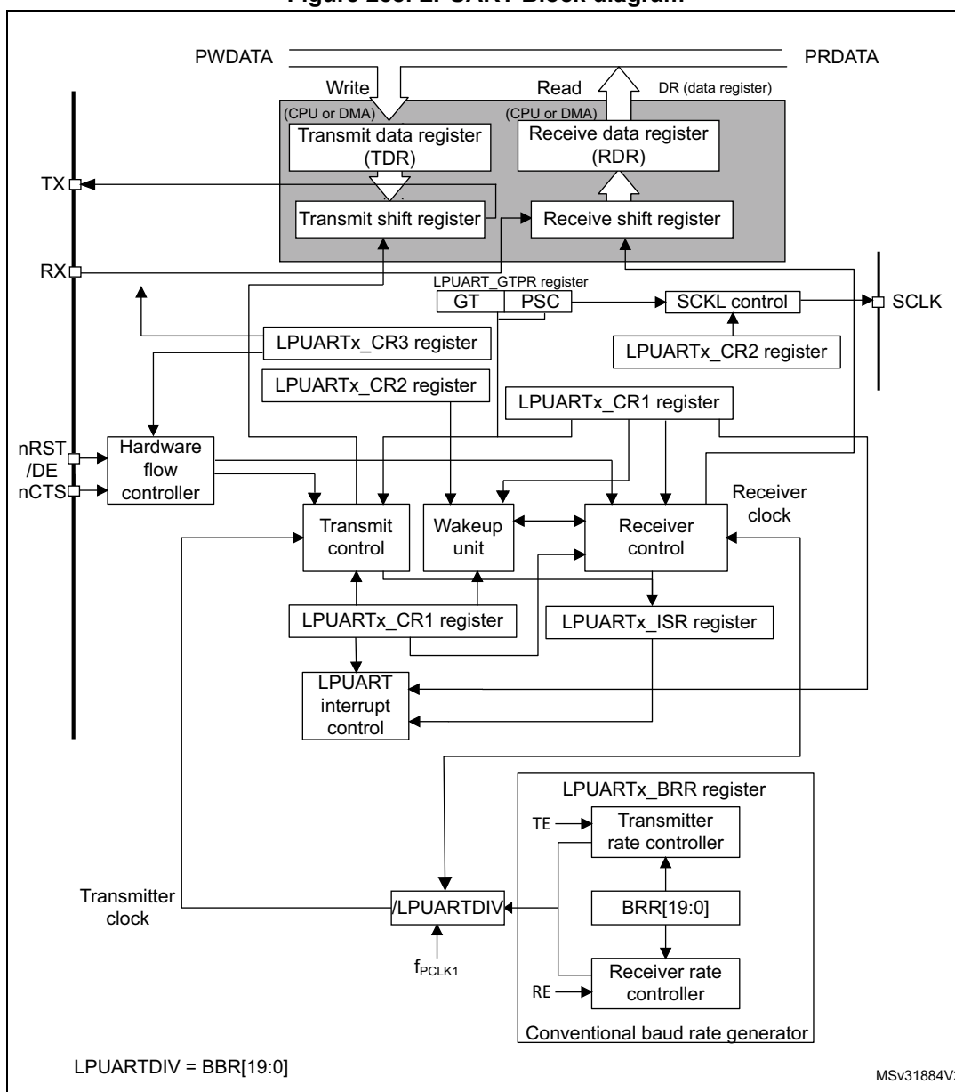
Figure 258. LPUART Block diagram
