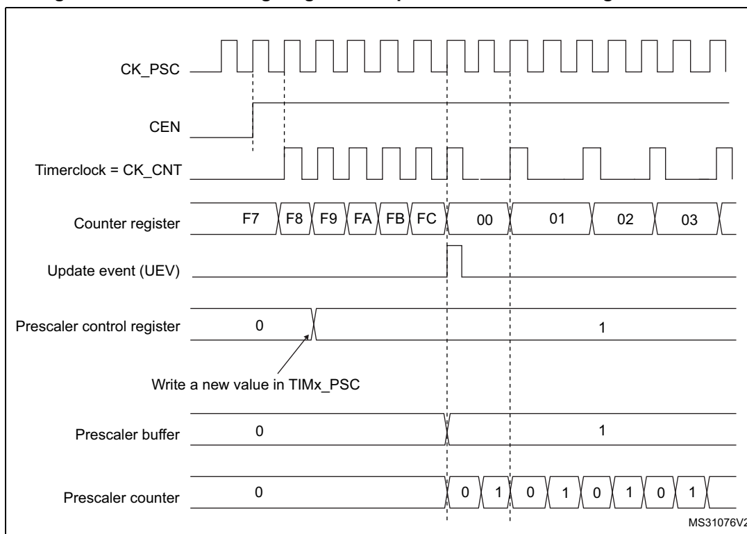
Figure 100. Counter timing diagram with prescaler division change from 1 to 2
