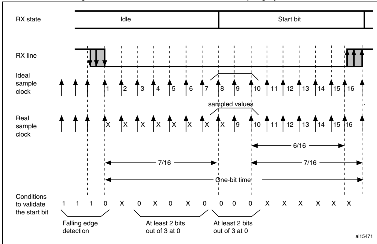
Figure 237. Start bit detection when oversampling by 16 or 8
