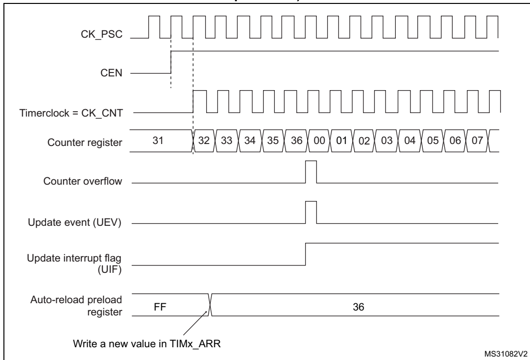
Figure 152. Counter timing diagram, update event when ARPE=0 (TIMx_ARR not preloaded)
