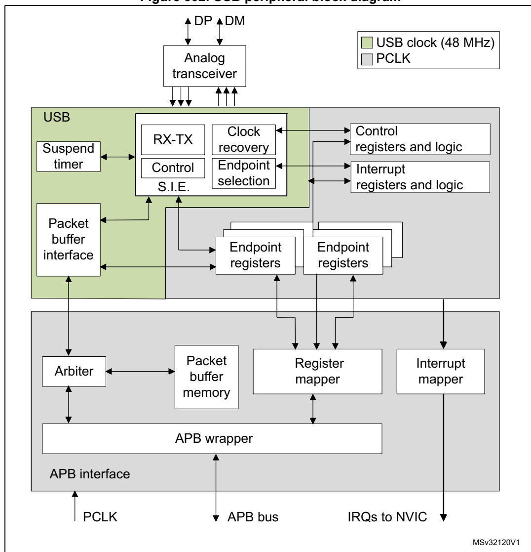
Figure 302. USB peripheral block diagram
