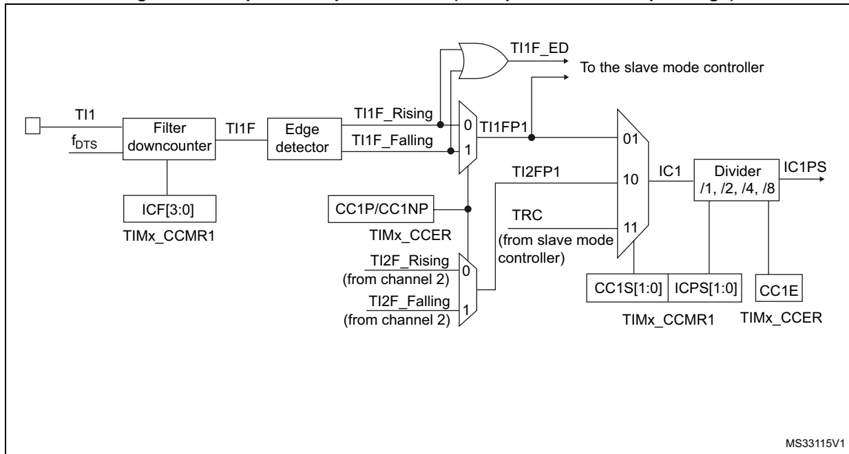
Figure 124. Capture/compare channel (example: channel 1 input stage)
