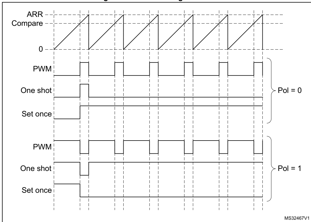
Figure 195. Waveform generation
