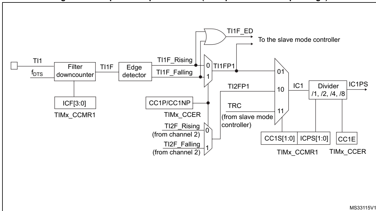
Figure 169. Capture/compare channel (example: channel 1 input stage)
