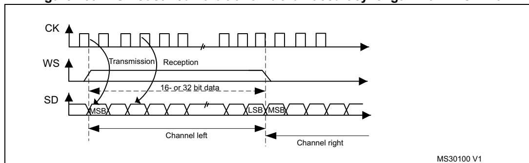
Figure 289. MSB Justified 16-bit or 32-bit full-accuracy length with CPOL = 0
