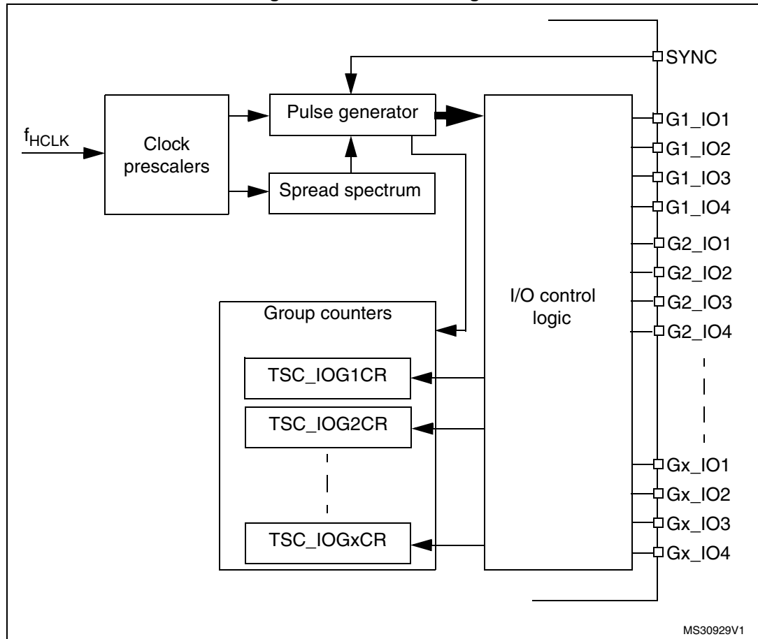
Figure 76. TSC block diagram
