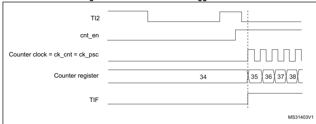
Figure 137. Control circuit in trigger mode
