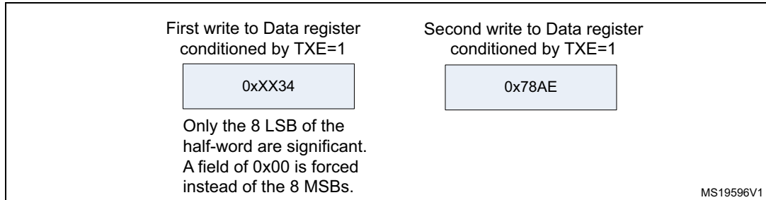
Figure 294. Operations required to transmit 0x3478AE
