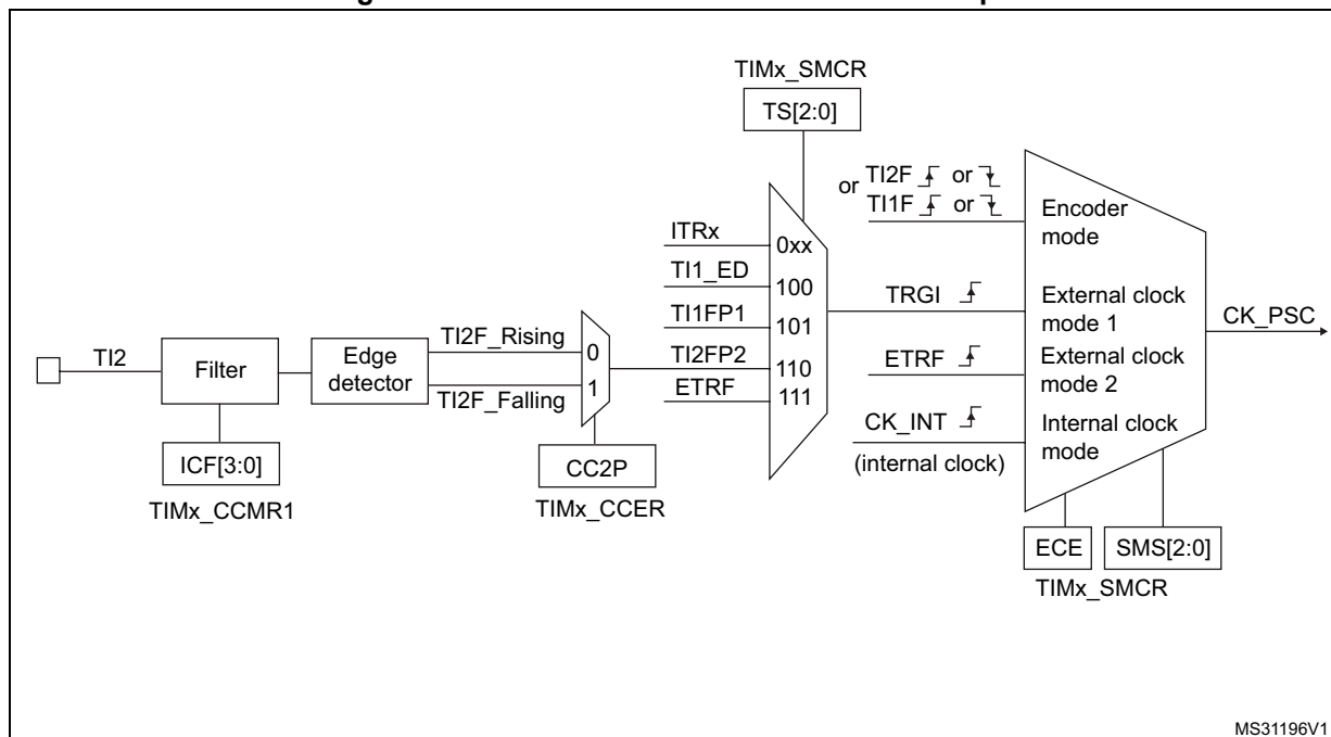
Figure 165. TI2 external clock connection example
