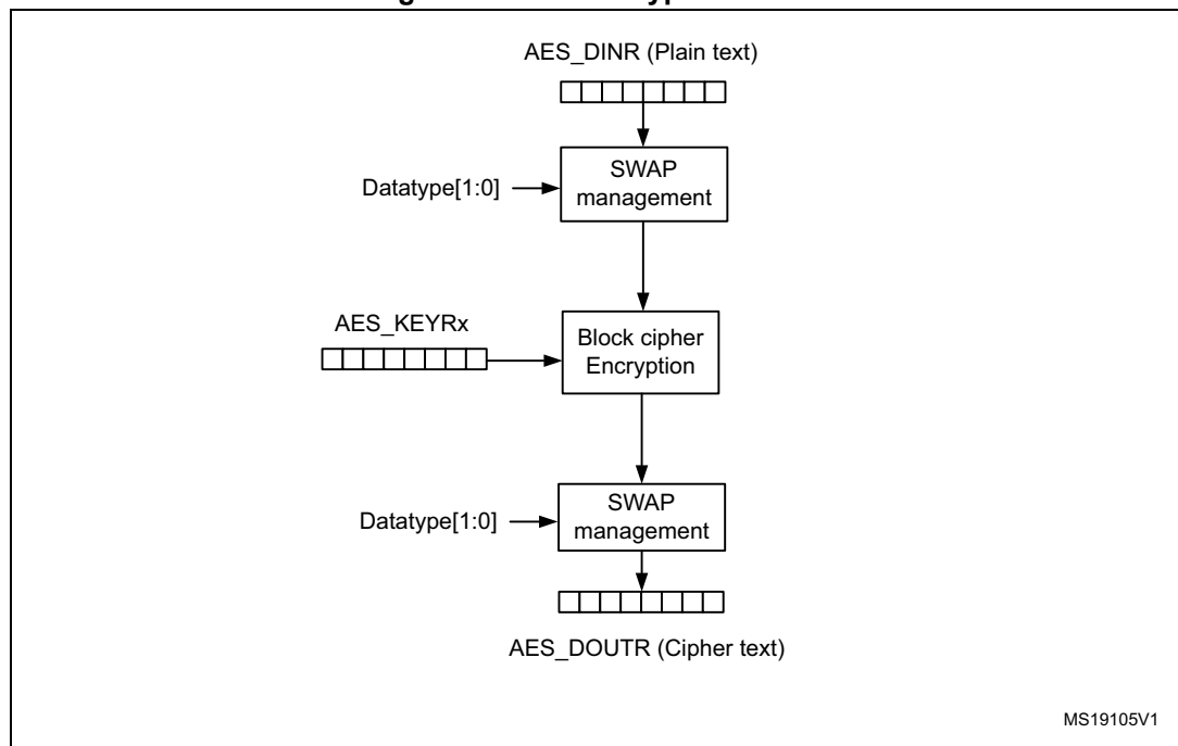
Figure 82. ECB encryption mode
