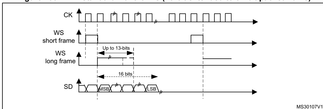
Figure 299. PCM standard waveforms (16-bit extended to 32-bit packet frame)
