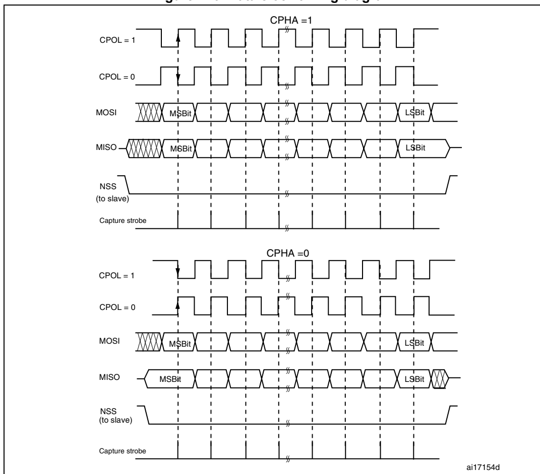
Figure 276. Data clock timing diagram
