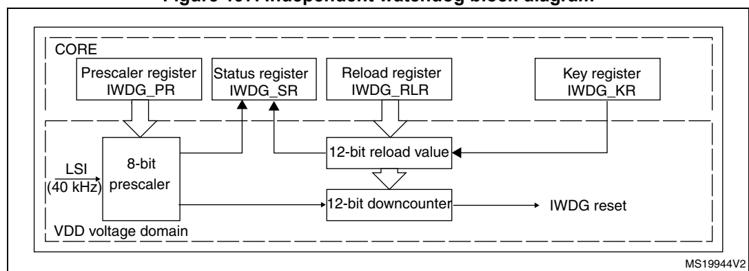
Figure 197. Independent watchdog block diagram
