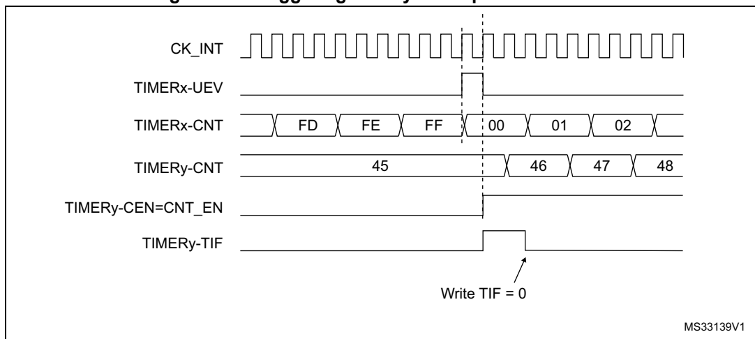
Figure 142. Triggering timer y with update of timer x
