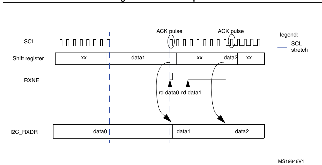
Figure 206. Data reception
