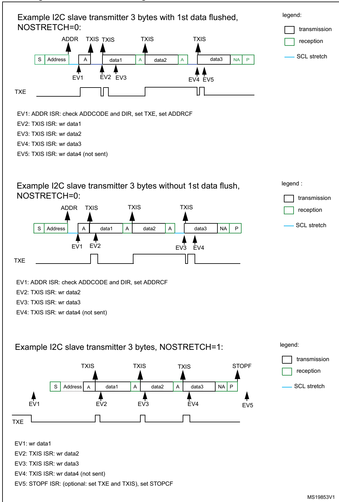
Figure 211. Transfer bus diagrams for I2C slave transmitter
