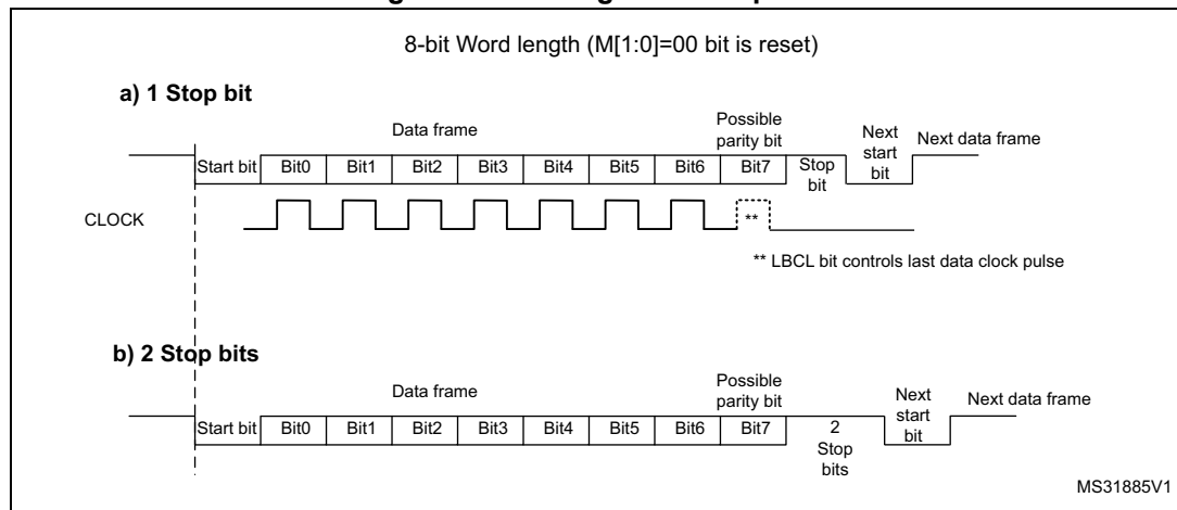
Figure 260. Configurable stop bits
