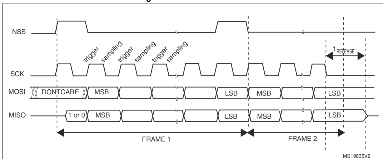
Figure 281. TI mode transfer
