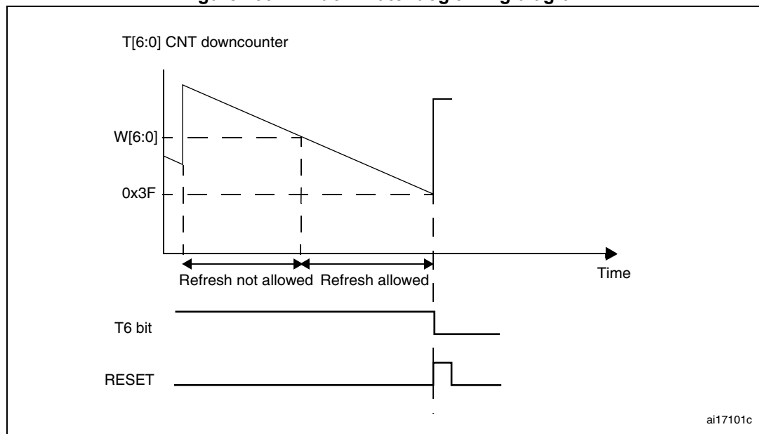
Figure 199. Window watchdog timing diagram
