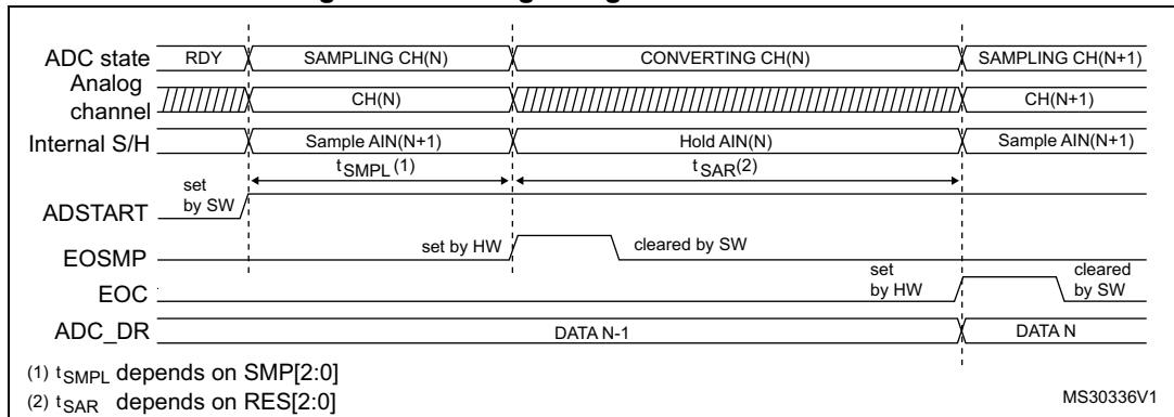
Figure 38. ADC conversion timings
