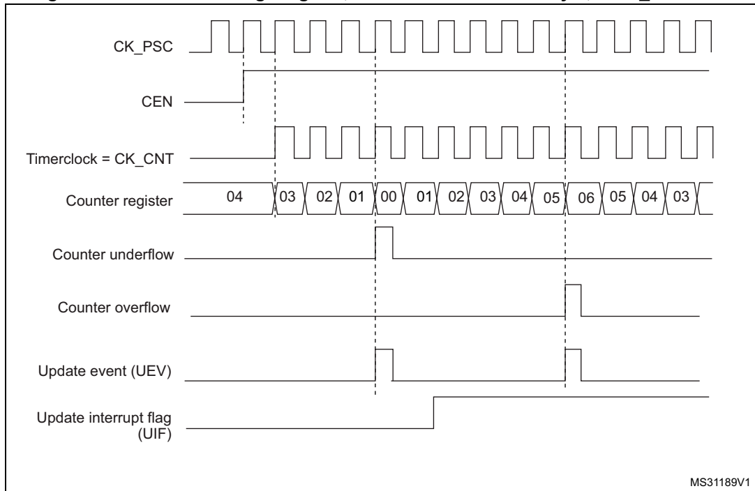
Figure 158. Counter timing diagram, internal clock divided by 1, TIMx_ARR=0x6
