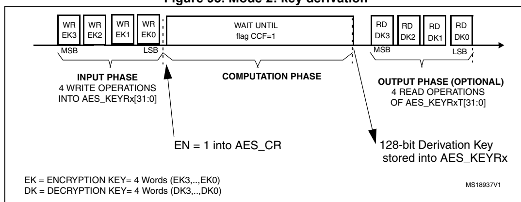
Figure 93. Mode 2: key derivation
