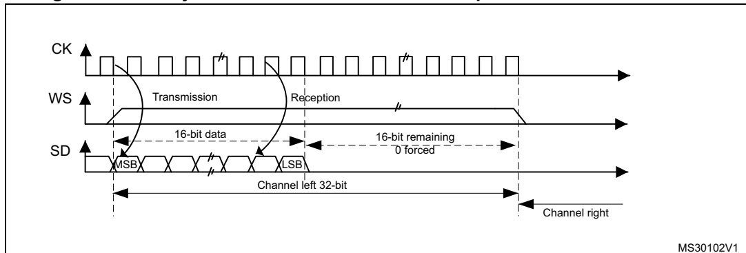
Figure 291. MSB justified 16-bit extended to 32-bit packet frame with CPOL = 0
