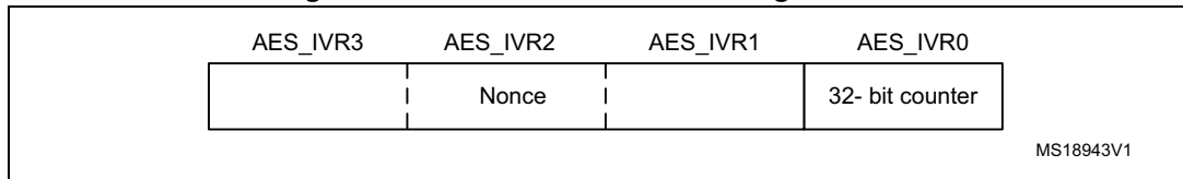
Figure 89. 32-bit counter + nonce organization
