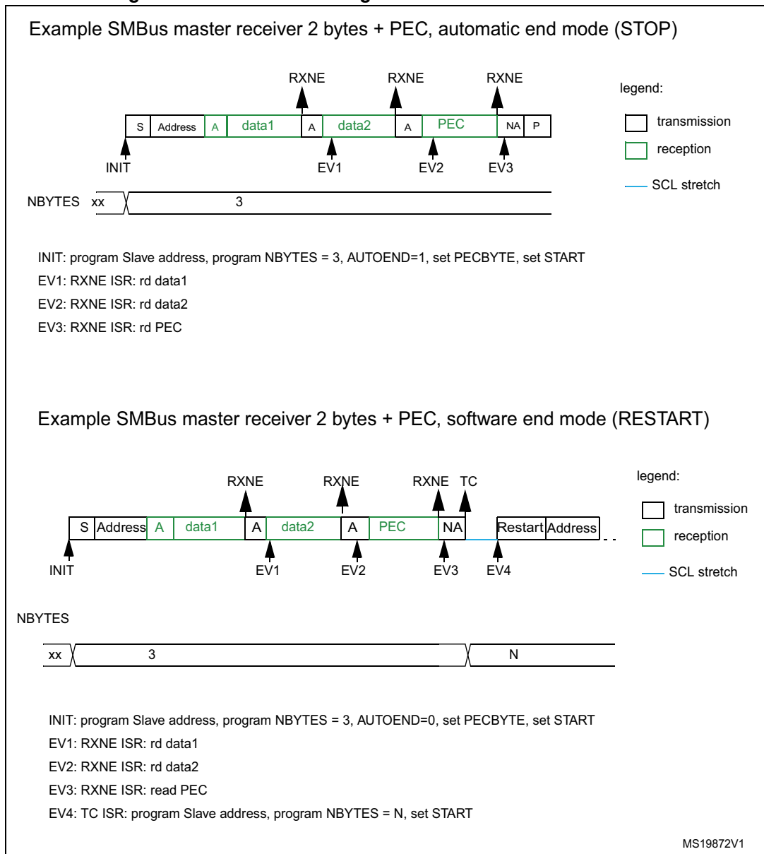
Figure 231. Bus transfer diagrams for SMBus master receiver
