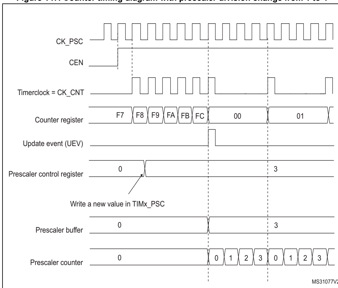
Figure 147. Counter timing diagram with prescaler division change from 1 to 4
