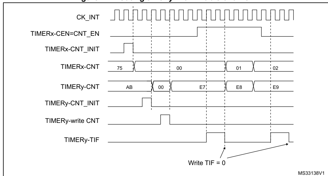
Figure 141. Gating timer y with Enable of timer x
