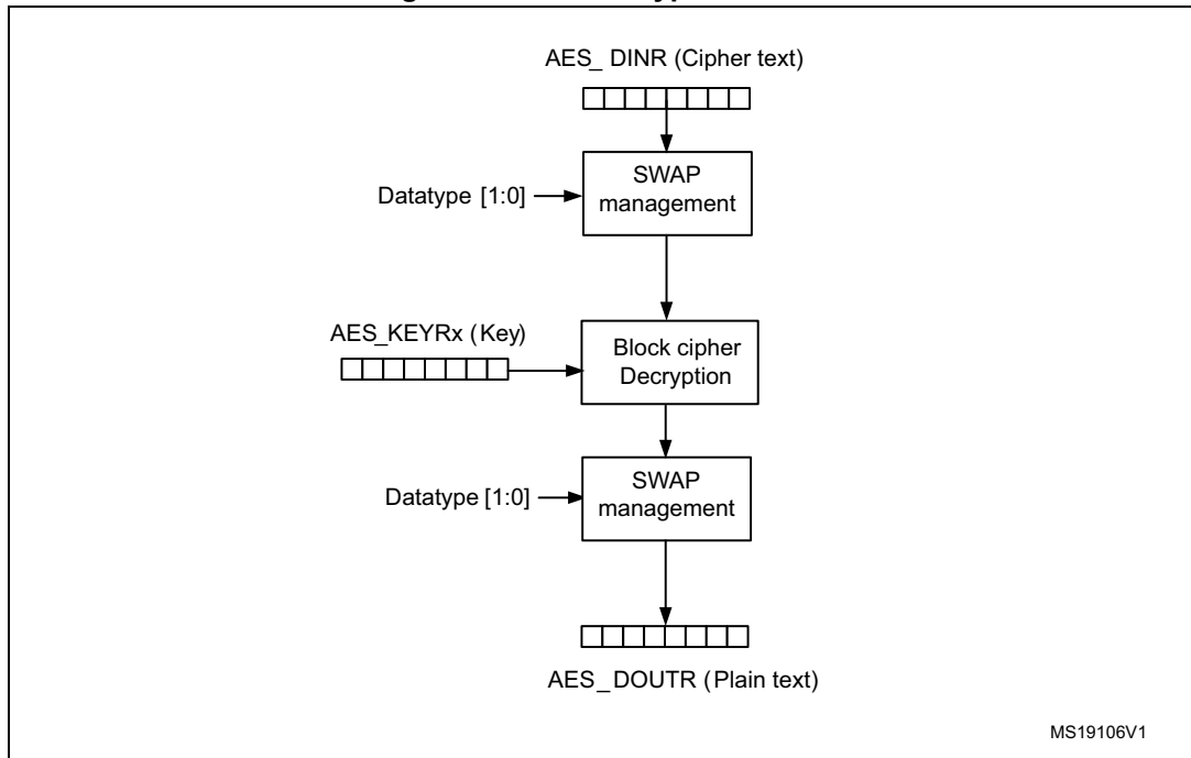
Figure 83. ECB decryption mode
