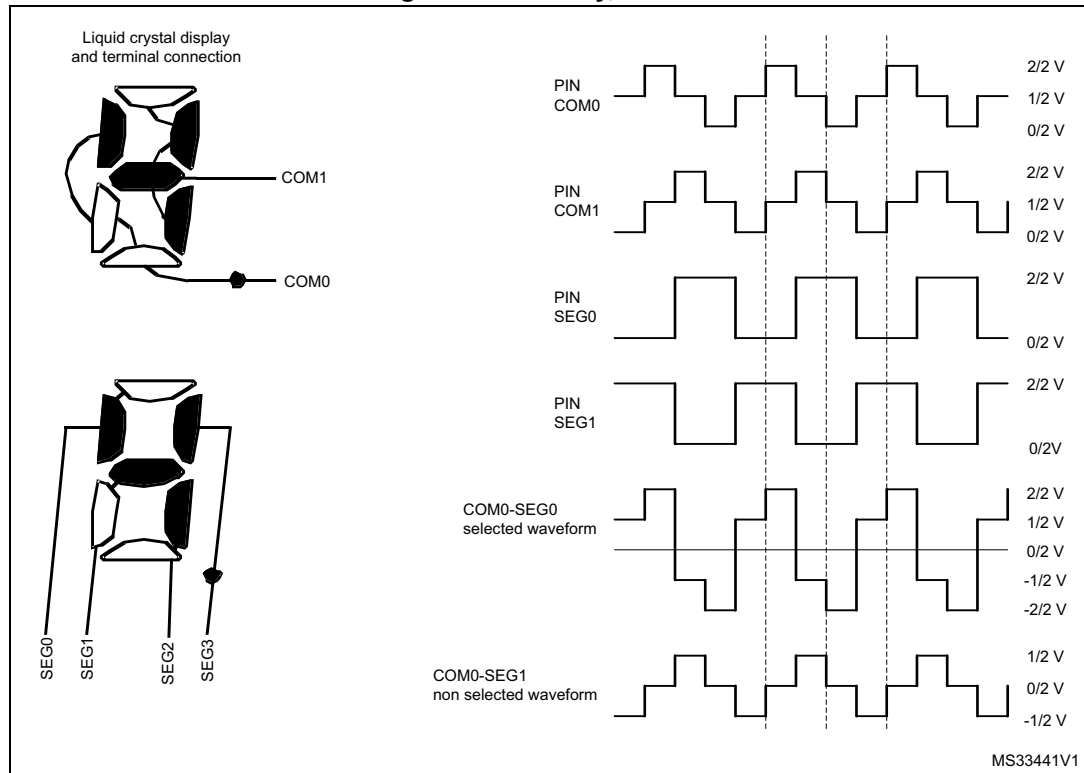
Figure 68. 1/2 duty, 1/2 bias
