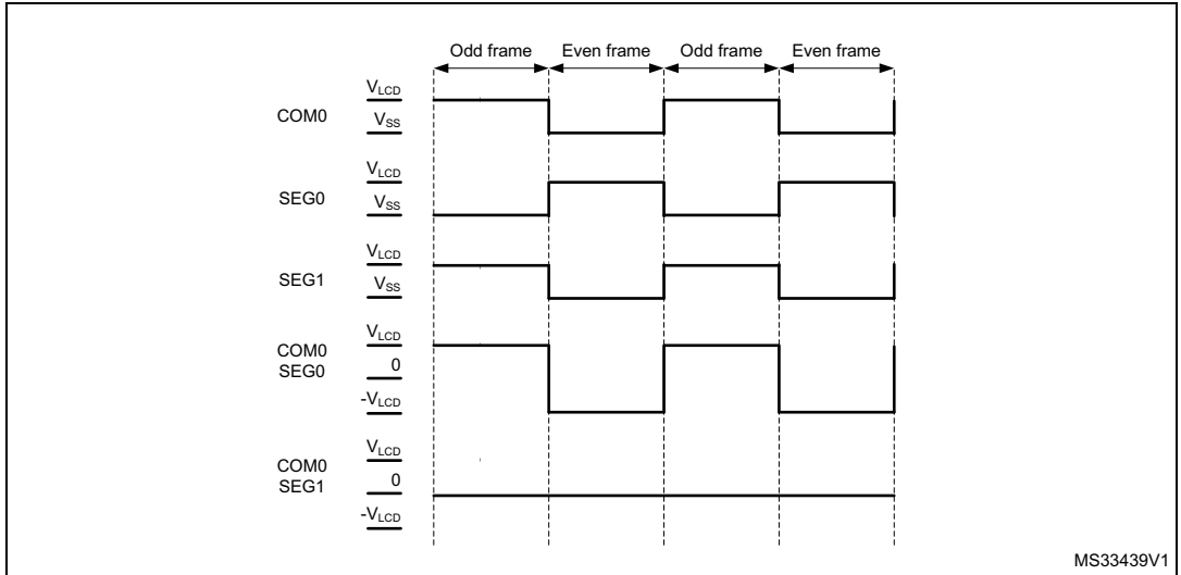
Figure 66. Static duty case 1
