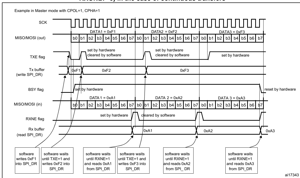
Figure 277. TXE/RXNE/BSY behavior in master / full-duplex mode (BIDIMODE=0, RXONLY=0) in the case of continuous transfers
