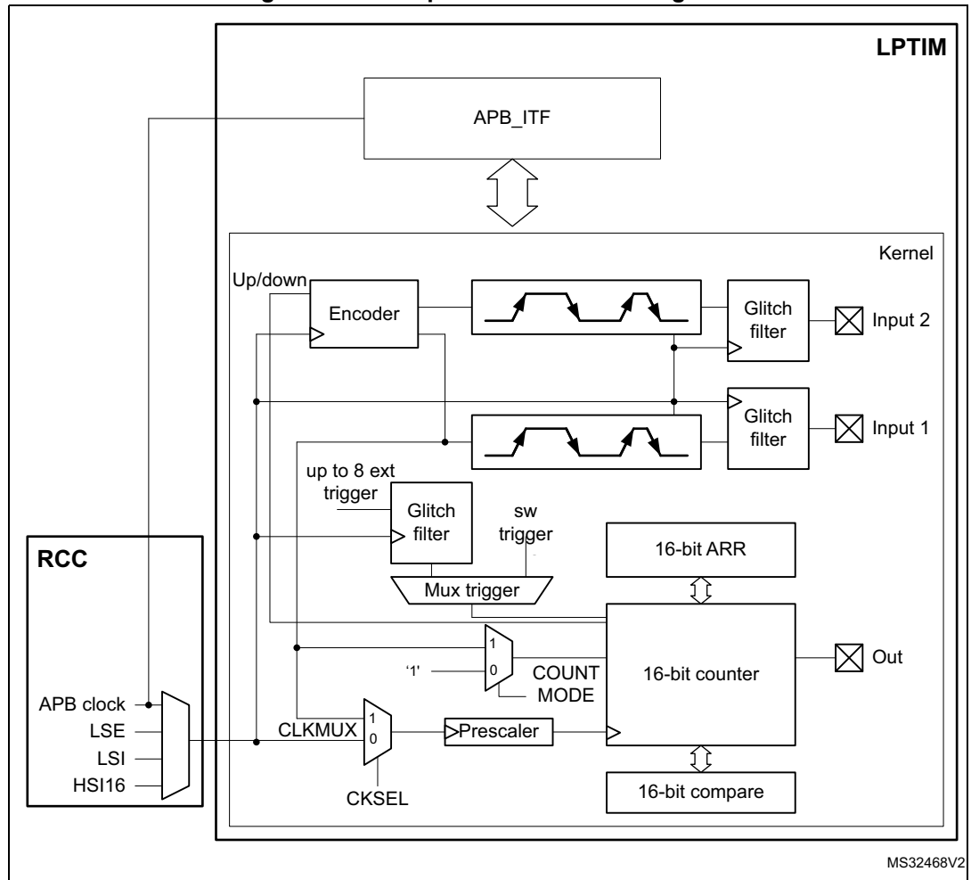
Figure 193. Low-power timer block diagram-
