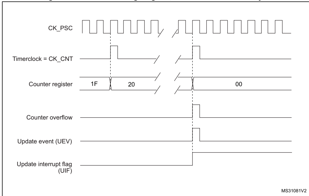
Figure 152. Counter timing diagram, update event when ARPE=0 (TIMx_ARR not preloaded)
