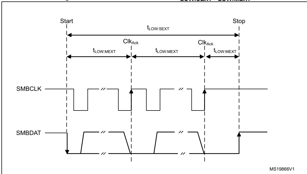
Figure 225. Timeout intervals for t_{\text{LOW:SEXT}} , t_{\text{LOW:MEXT}}
