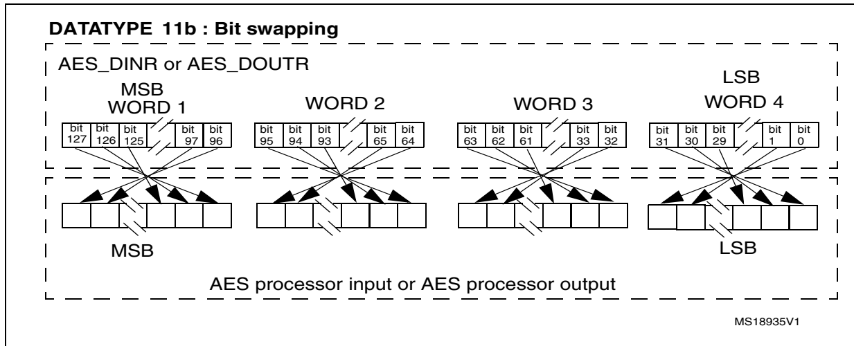
Figure 91. 128-bit block construction according to the data type (continued)
