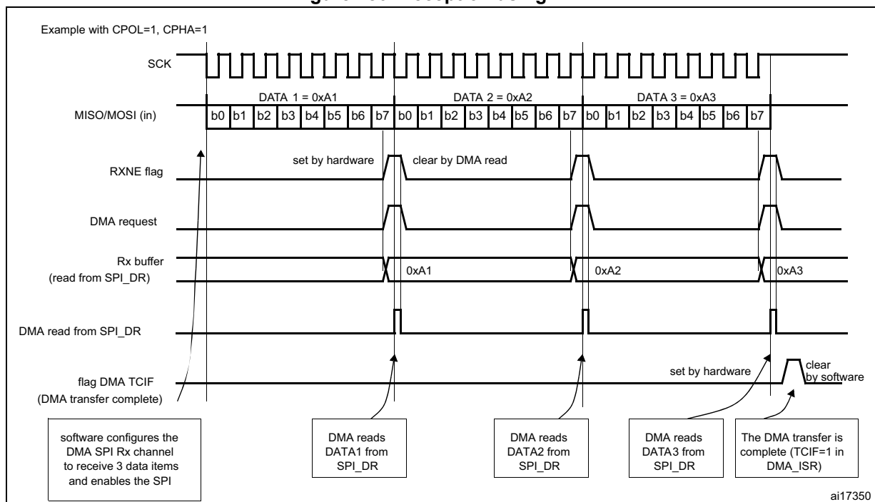
Figure 280. Reception using DMA
