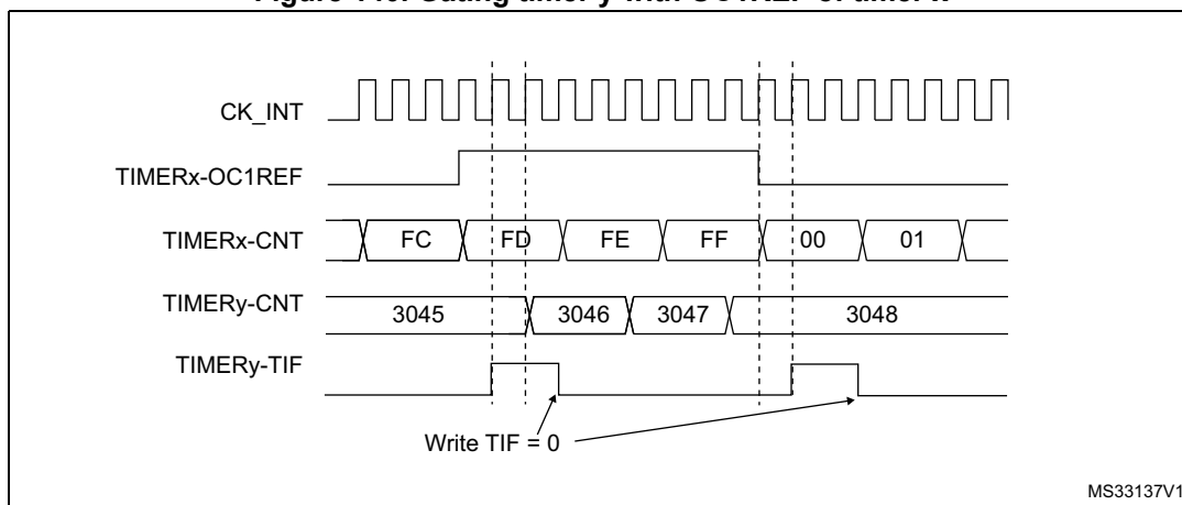
Figure 140. Gating timer y with OC1REF of timer x
