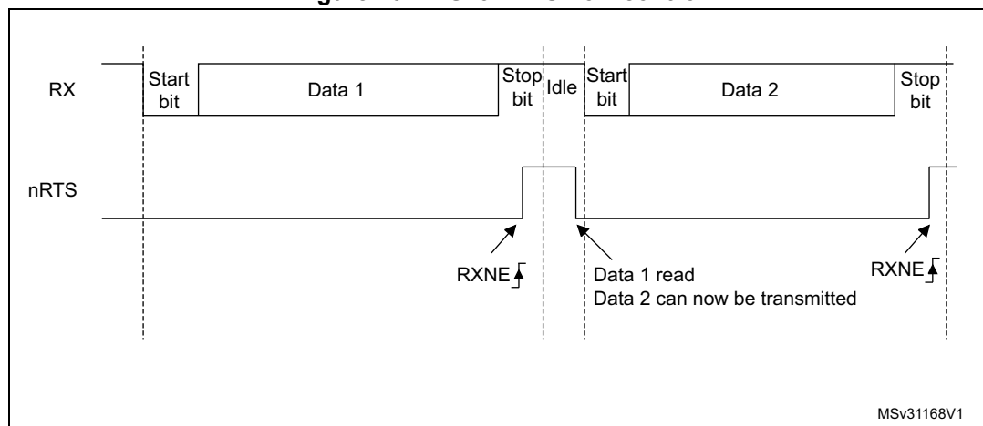
Figure 267. RS232 RTS flow control
