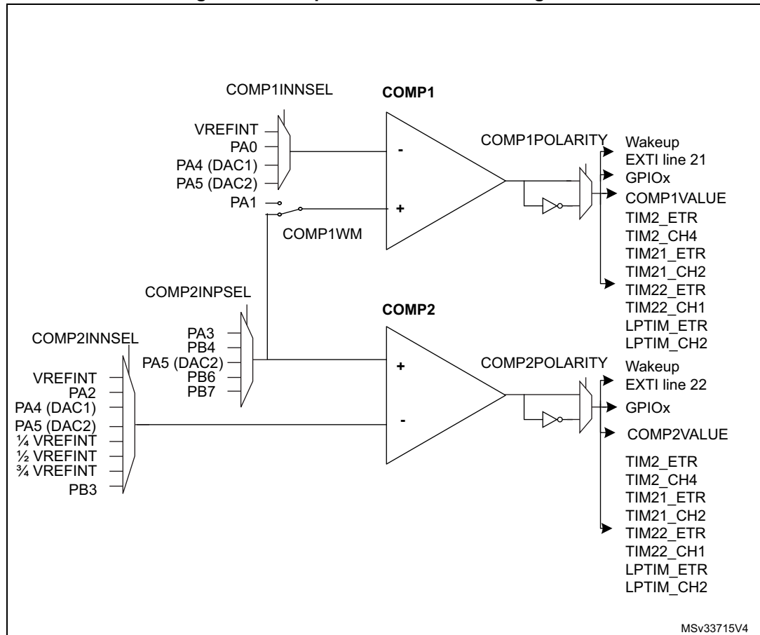
Figure 63. Comparator 1 and 2 block diagrams
