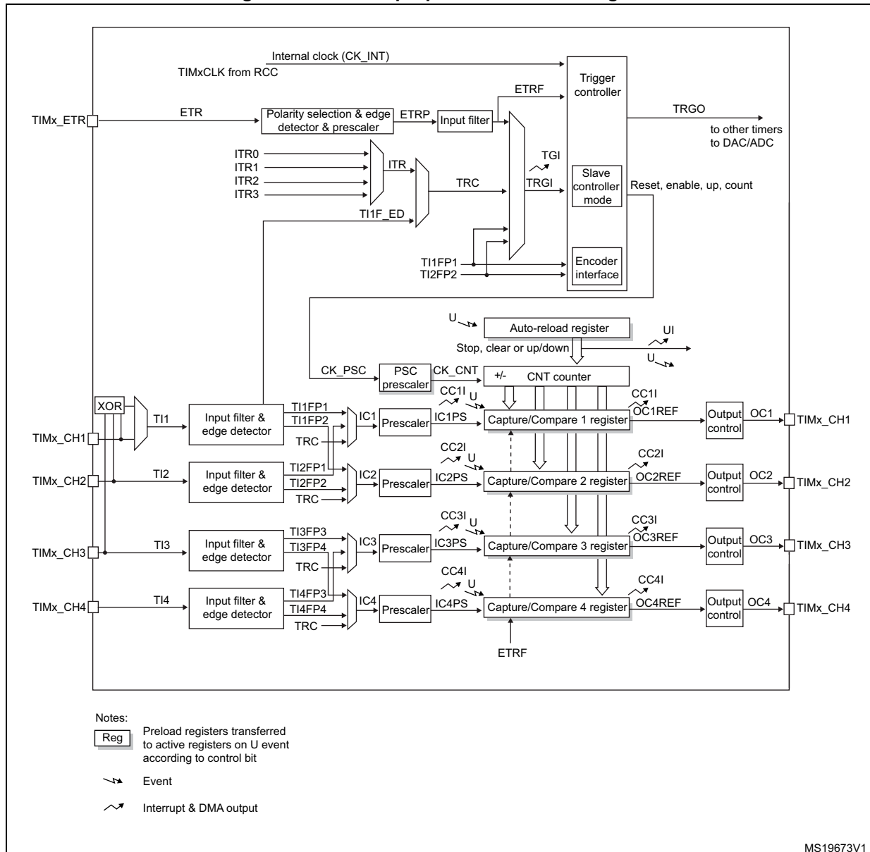
Figure 99. General-purpose timer block diagram
