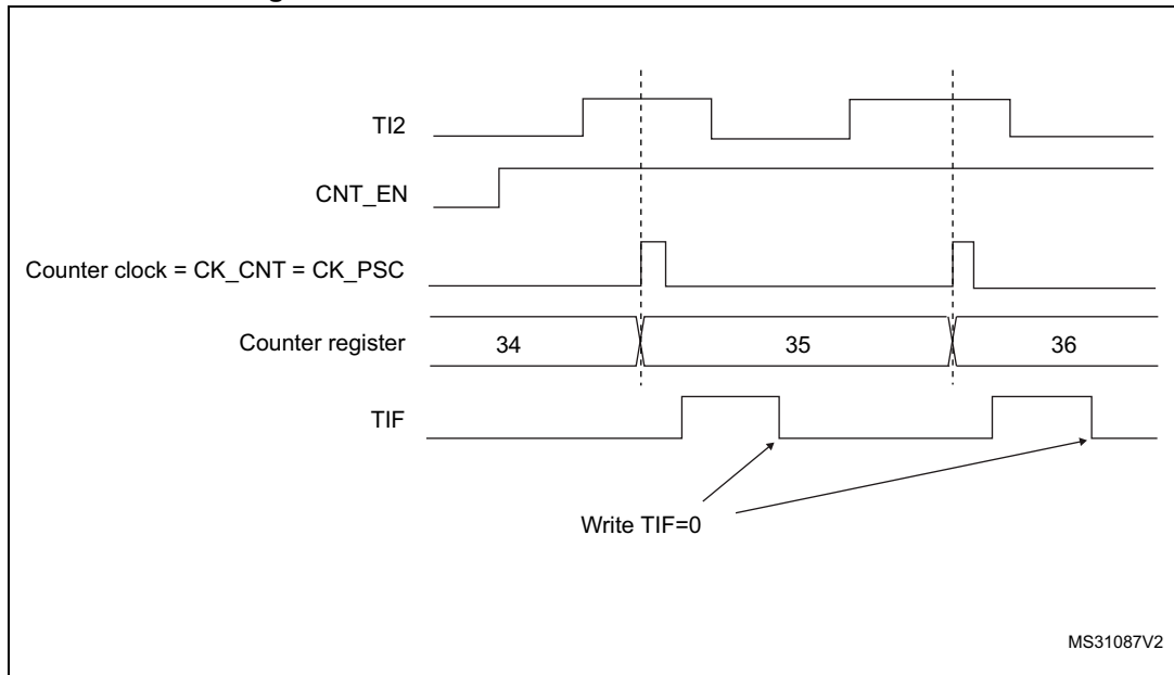
Figure 166. Control circuit in external clock mode 1
