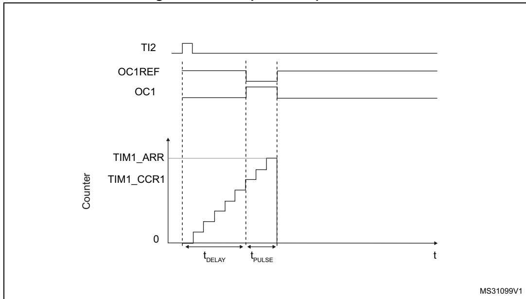
Figure 177. Example of one pulse mode
