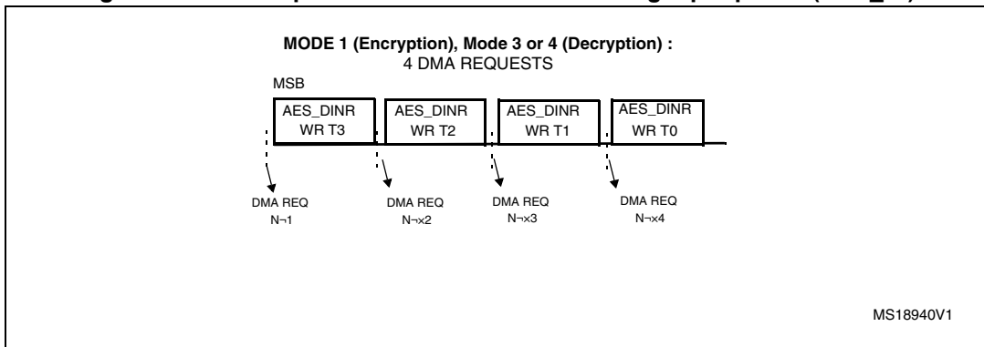
Figure 96. DMA requests and data transfers during Input phase (AES_IN)
