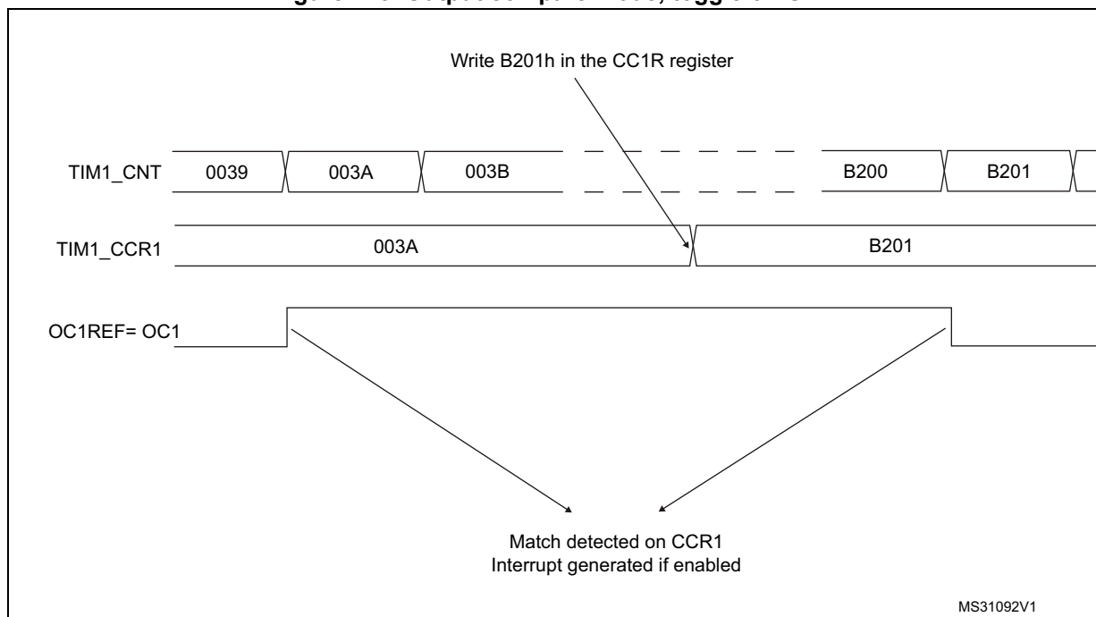
Figure 128. Output compare mode, toggle on OC1.
