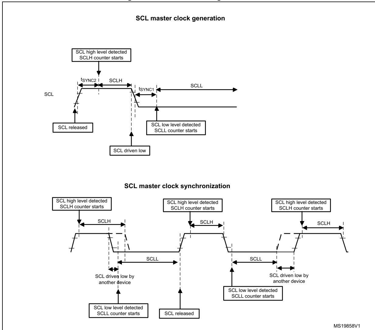
Figure 215. Master clock generation
