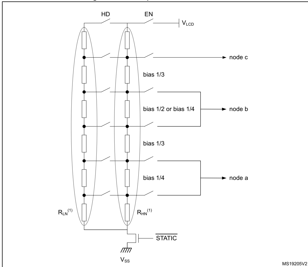
Figure 72. VLCD pin for 1/2 1/3 1/4 bias
