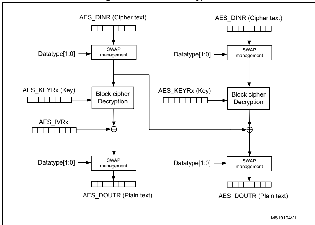
Figure 85. CBC mode decryption
