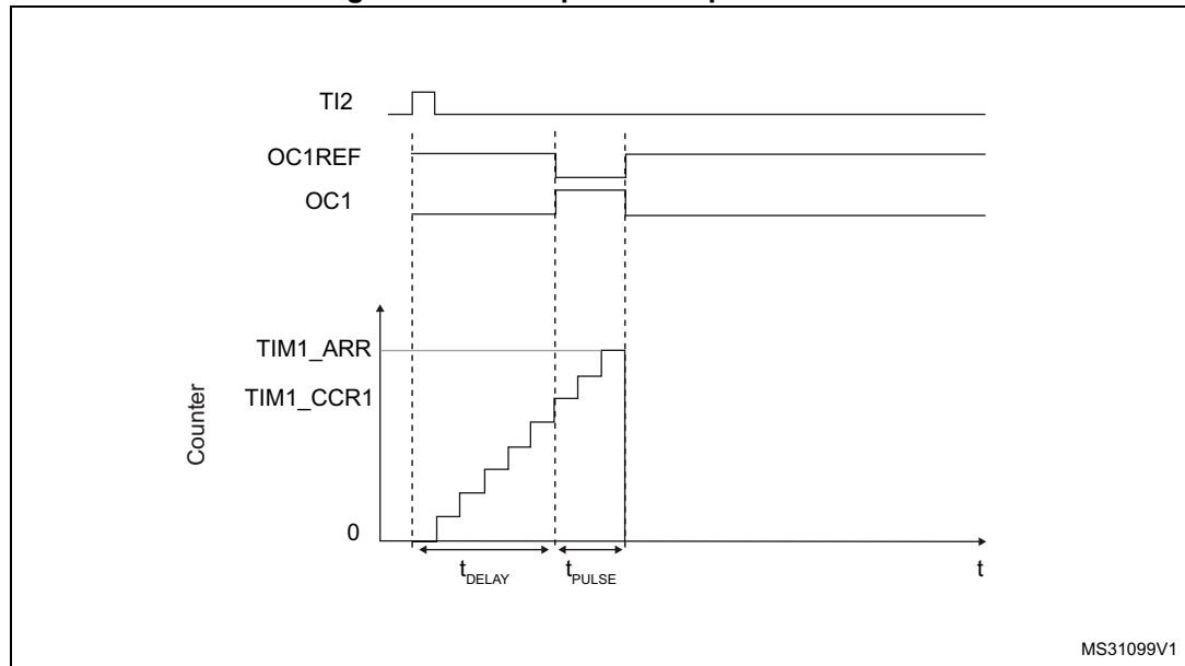
Figure 131. Example of one-pulse mode.
