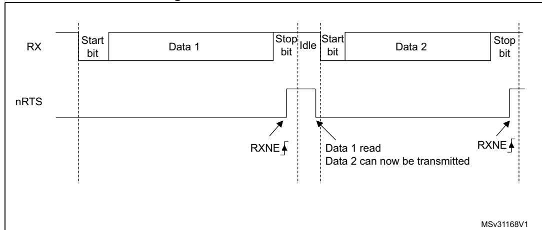
Figure 255. RS232 RTS flow control
