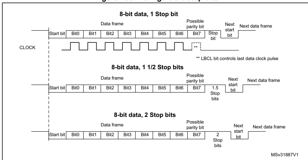
Figure 235. Configurable stop bits
