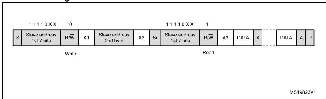
Figure 217. 10-bit address read access with HEAD10R=0
