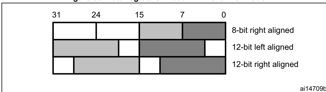
Figure 58. Data registers in dual DAC channel mode
