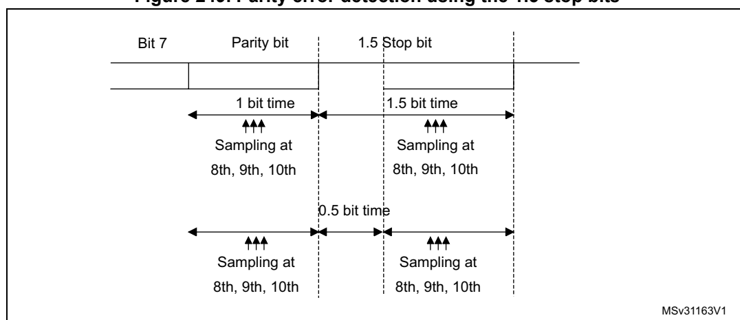
Figure 249. Parity error detection using the 1.5 stop bits
