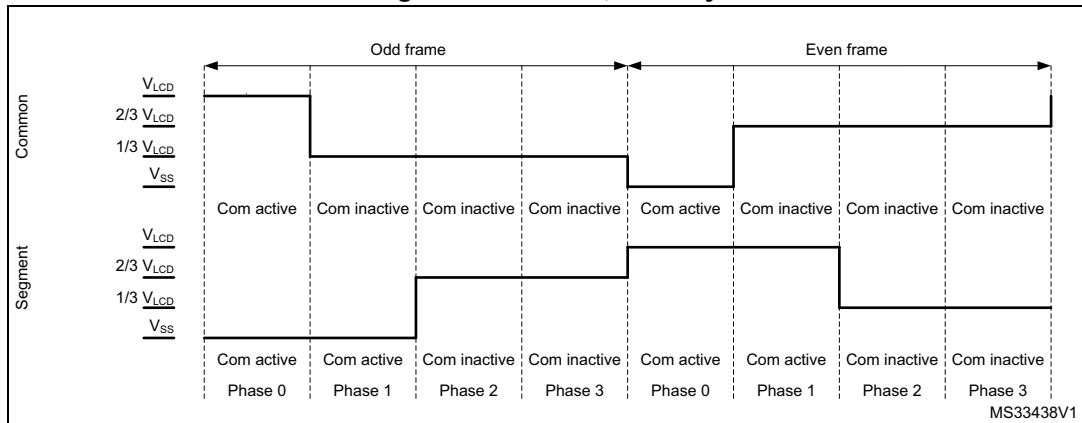
Figure 65. 1/3 bias, 1/4 duty
