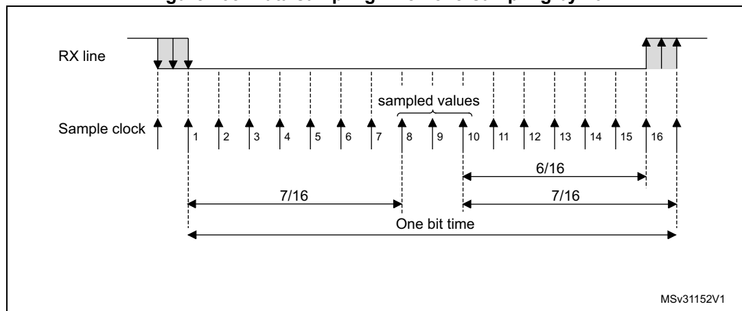
Figure 238. Data sampling when oversampling by 16
