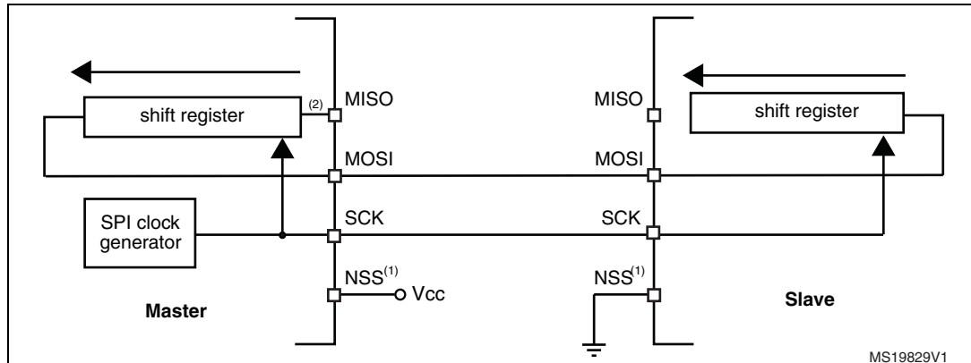
Figure 273. Simplex single master/single slave application (master in transmit-only/ slave in receive-only mode)
