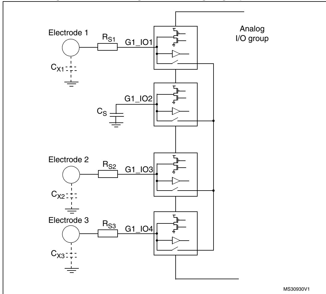
Figure 77. Surface charge transfer analog I/O group structure
