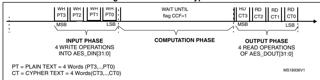
Figure 92. Mode 1: encryption
