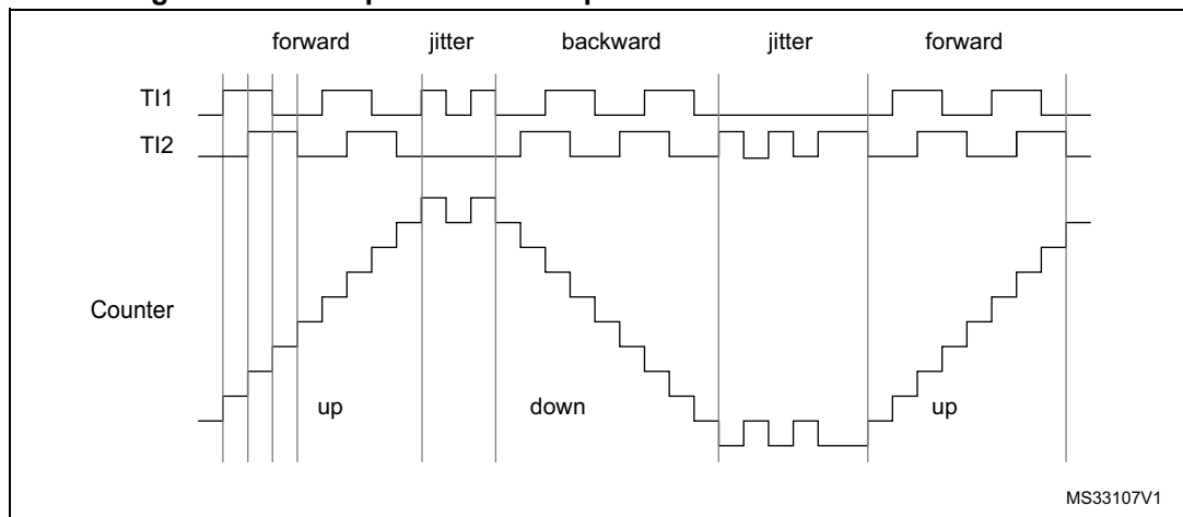
Figure 178. Example of counter operation in encoder interface mode
