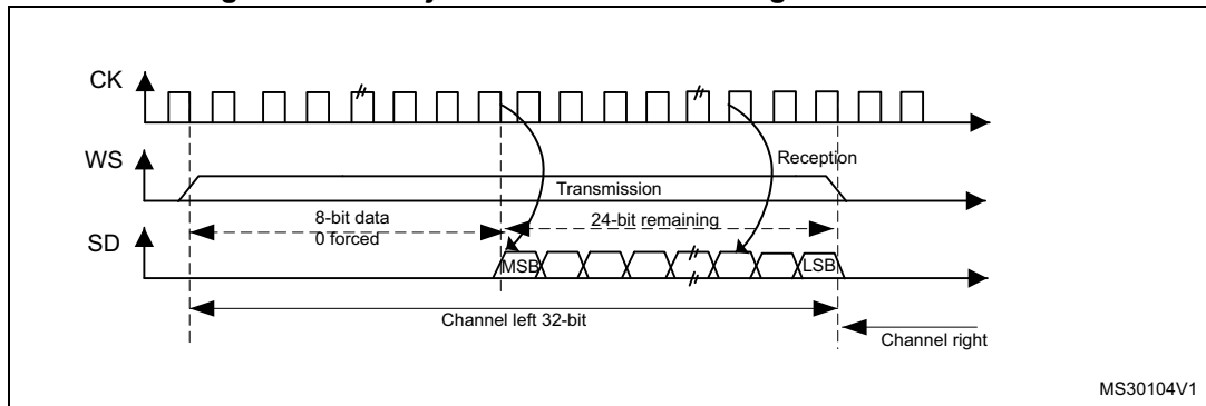
Figure 293. LSB justified 24-bit frame length with CPOL = 0
