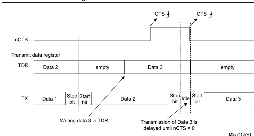
Figure 256. RS232 CTS flow control
