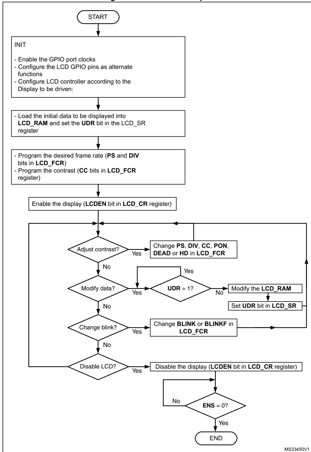
Figure 75. Flowchart example
