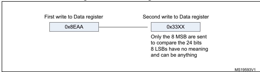
Figure 285. Transmitting 0x8EAA33
