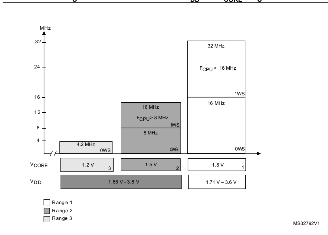
Figure 11. Performance versus V DD and V CORE range
