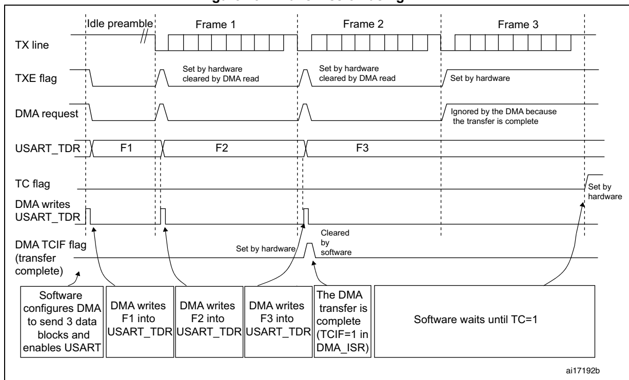
Figure 252. Transmission using DMA
