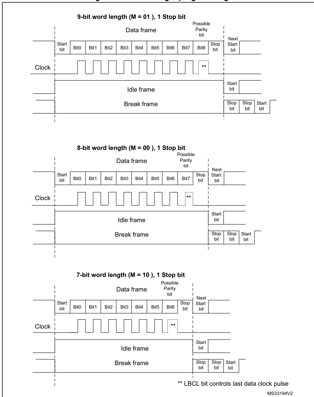
Figure 234. Word length programming
