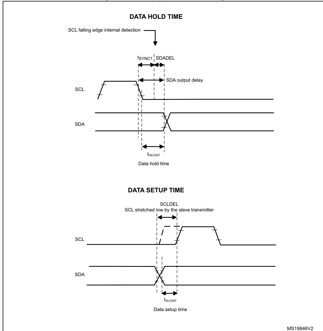
Figure 204. Setup and hold timings
