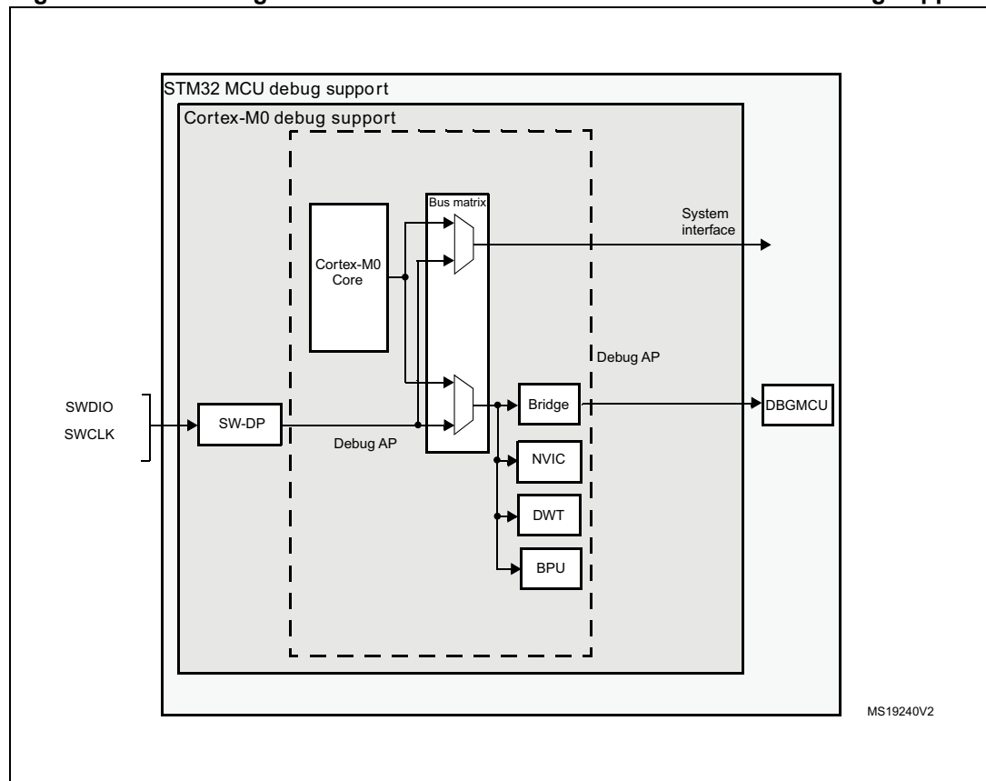
Figure 304. Block diagram of STM32L0x3 MCU and Cortex®-M0+-level debug support
