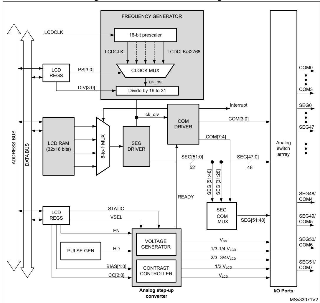
Figure 64. LCD controller block diagram
