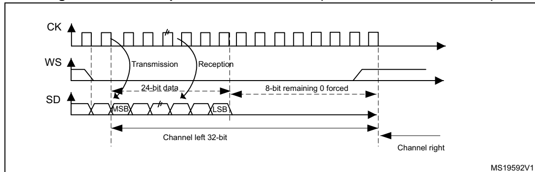
Figure 284. I 2 S Philips standard waveforms (24-bit frame with CPOL = 0)
