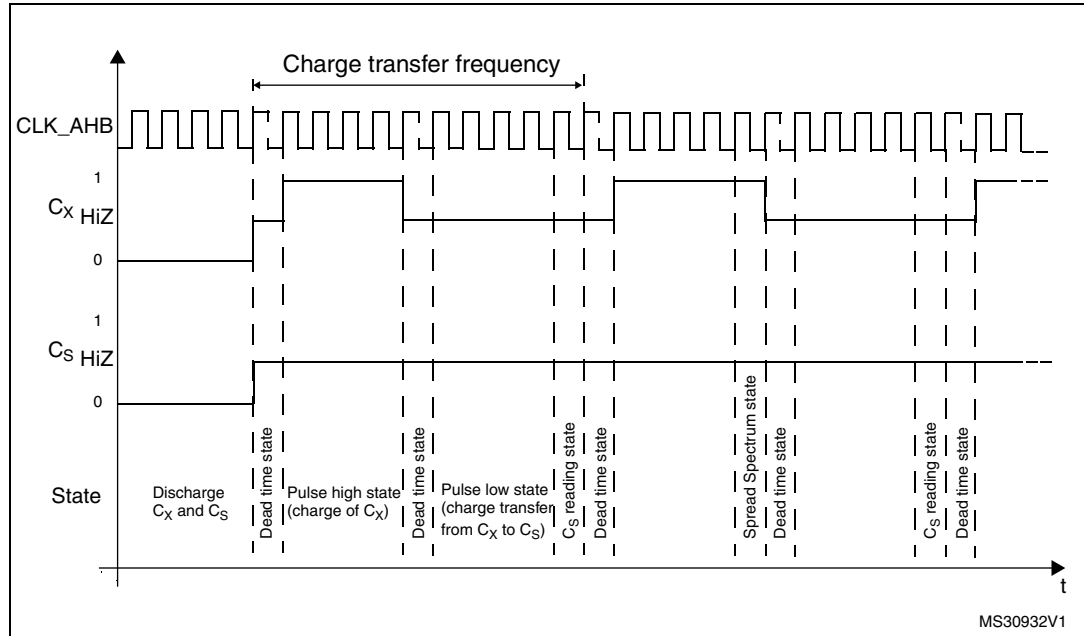
Figure 79. Charge transfer acquisition sequence
