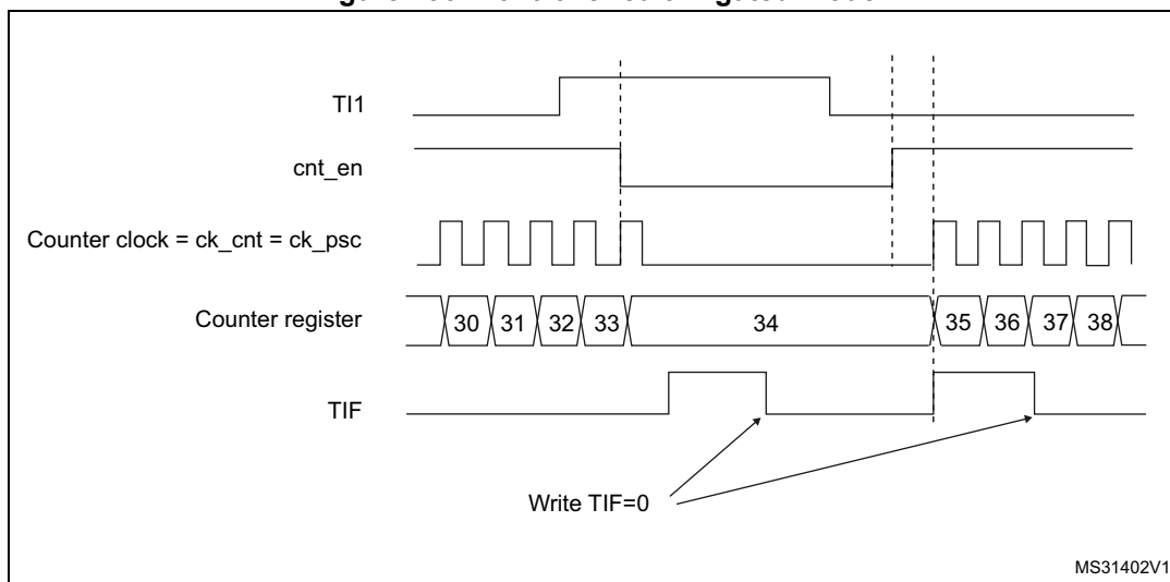
Figure 136. Control circuit in gated mode
