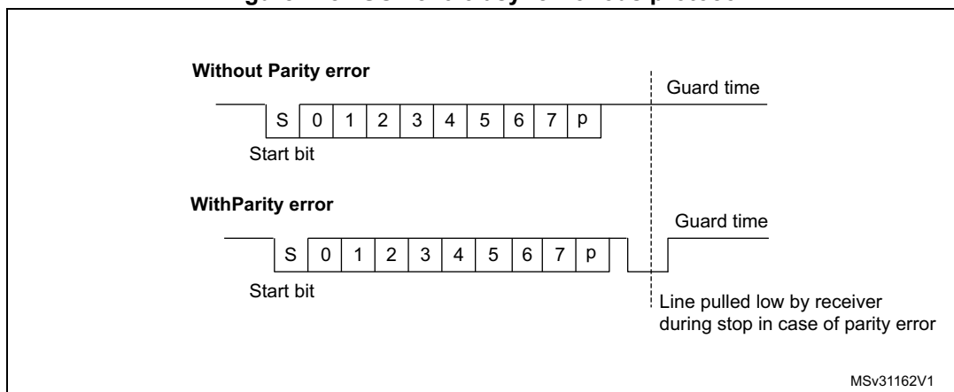
Figure 248. ISO 7816-3 asynchronous protocol
