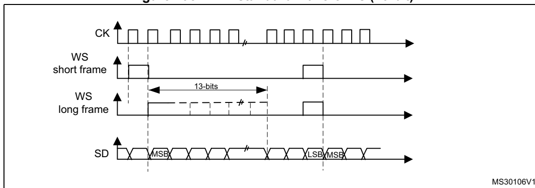
Figure 298. PCM standard waveforms (16-bit)
