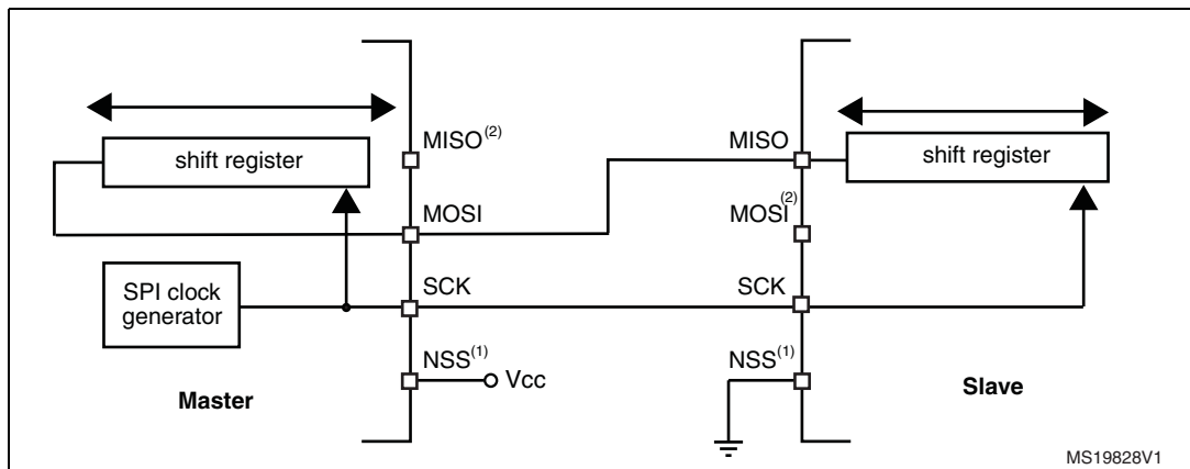
Figure 272. Half-duplex single master/ single slave application
