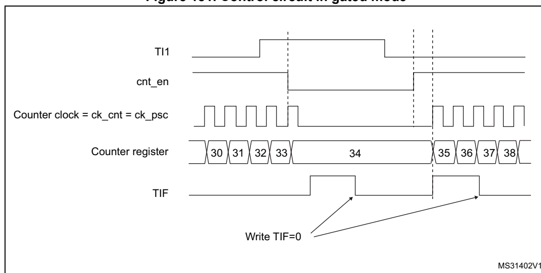
Figure 181. Control circuit in gated mode
