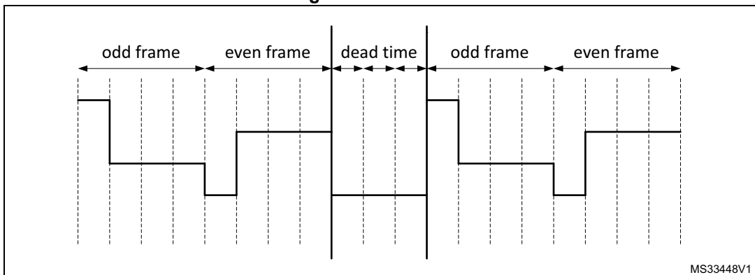
Figure 73. Deadtime
