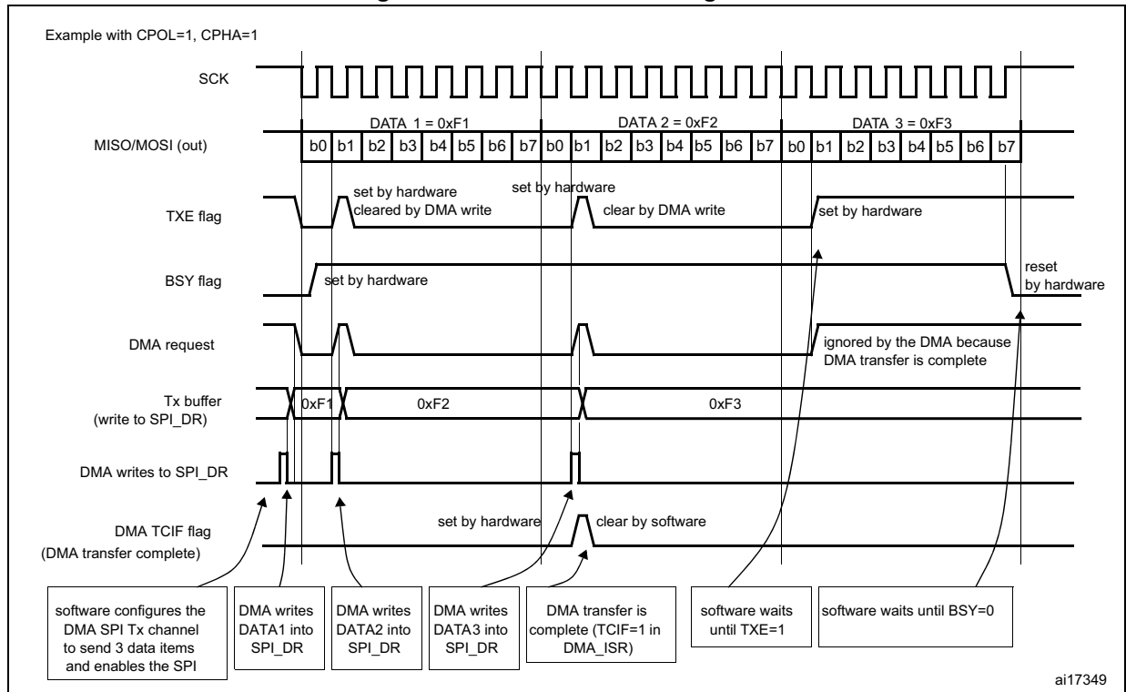
Figure 279. Transmission using DMA
