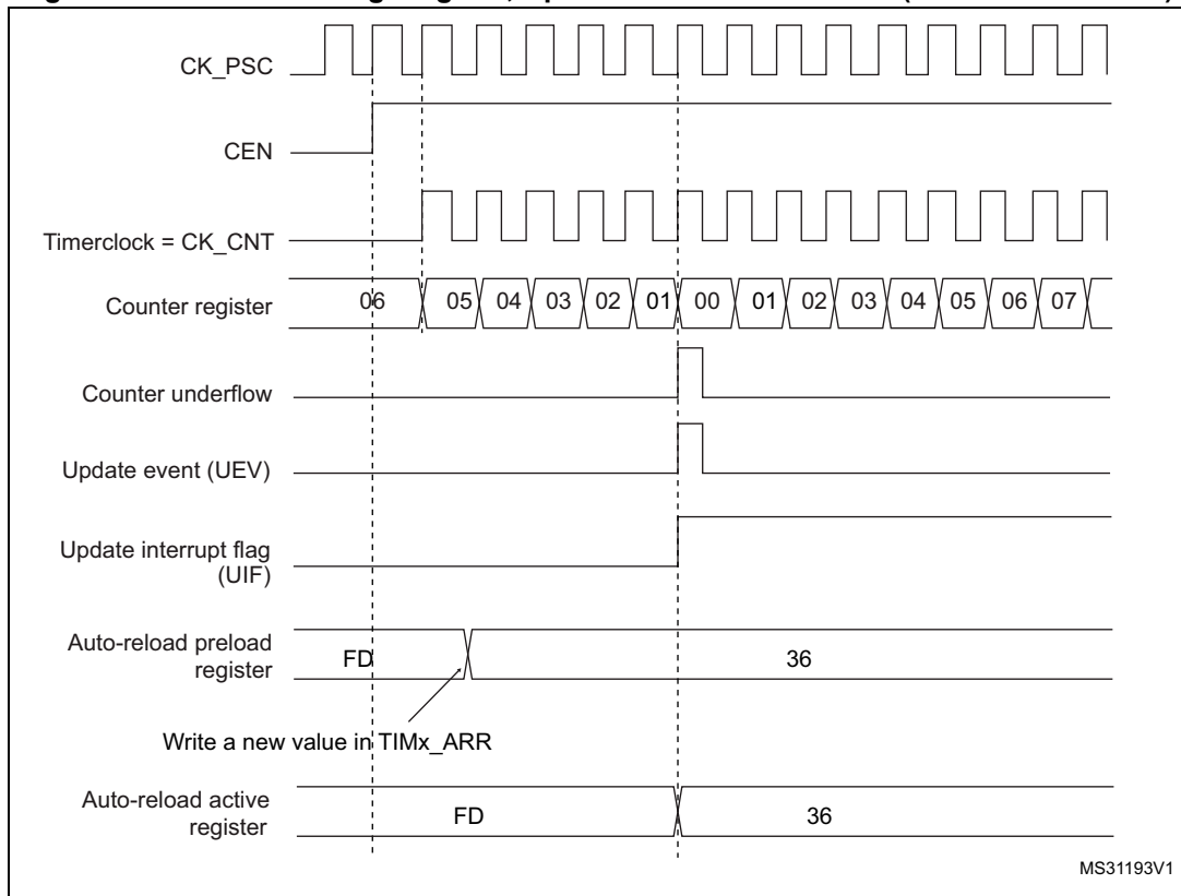
Figure 117. Counter timing diagram, Update event with ARPE=1 (counter underflow)
