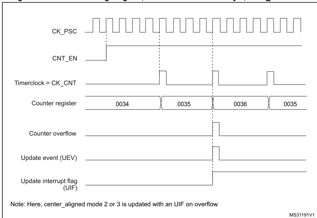
Figure 115. Counter timing diagram, internal clock divided by 4, TIMx_ARR=0x36
