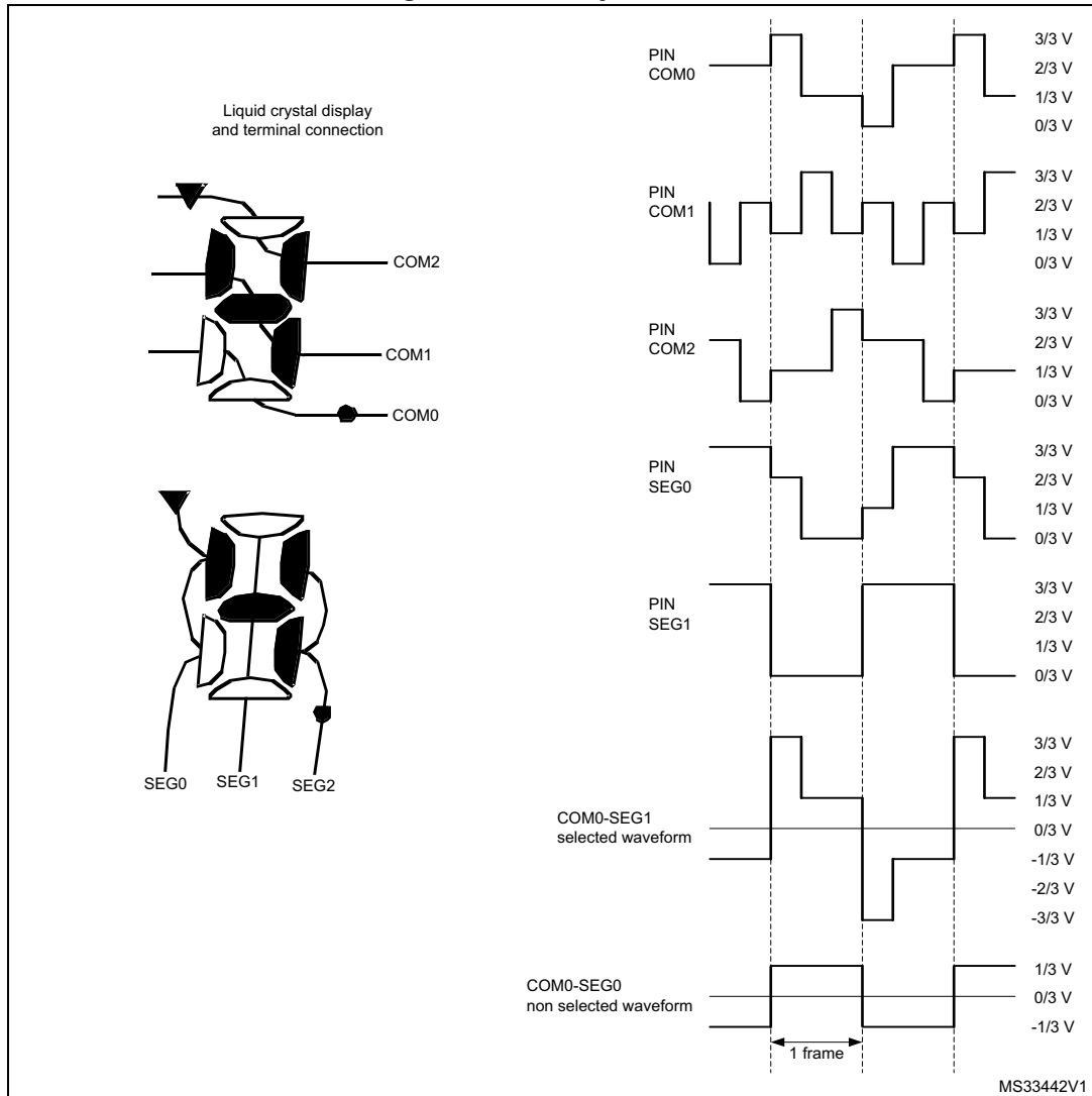
Figure 69. 1/3 duty, 1/3 bias
