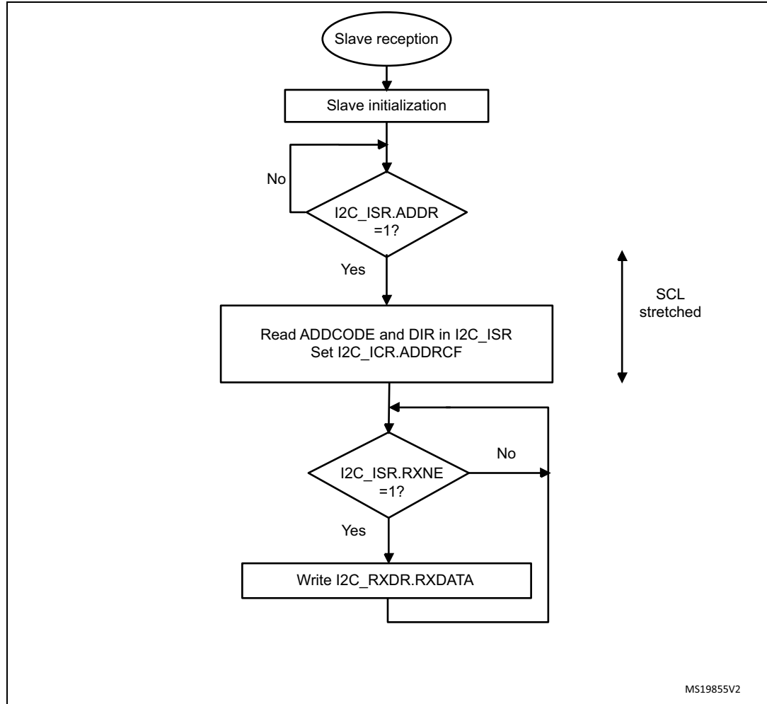
Figure 212. Transfer sequence flowchart for slave receiver with NOSTRETCH=0
