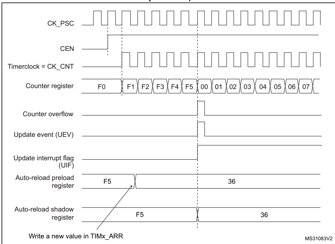
Figure 191. Counter timing diagram, update event when ARPE=1 (TIMx_ARR preloaded)
