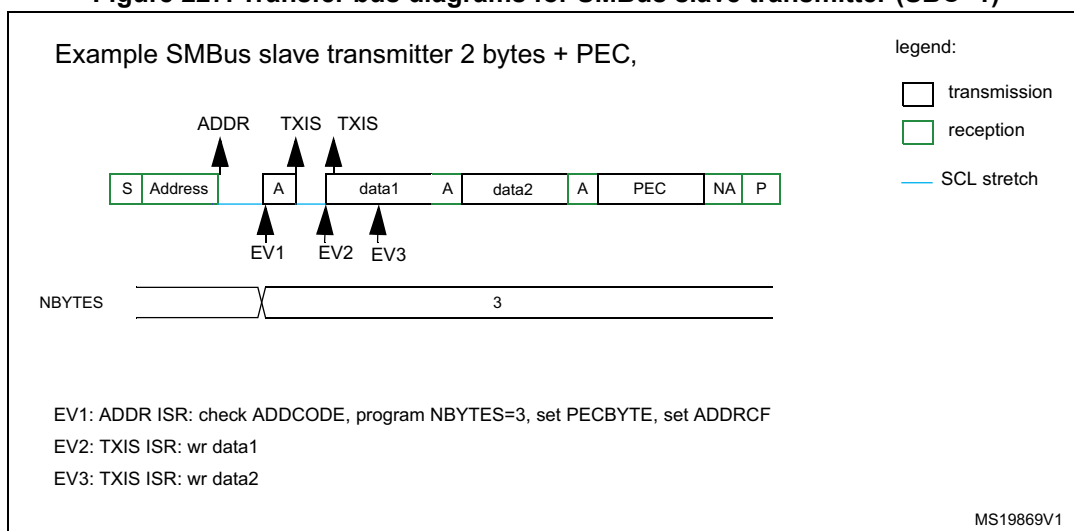
Figure 227. Transfer bus diagrams for SMBus slave transmitter (SBC=1)
