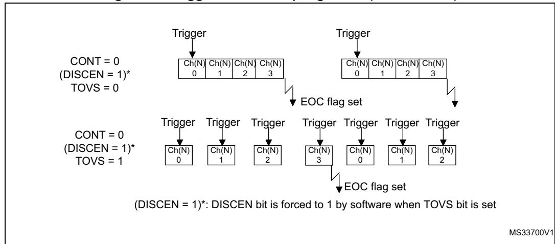
Figure 52. Triggered oversampling mode (TOVS bit = 1)
