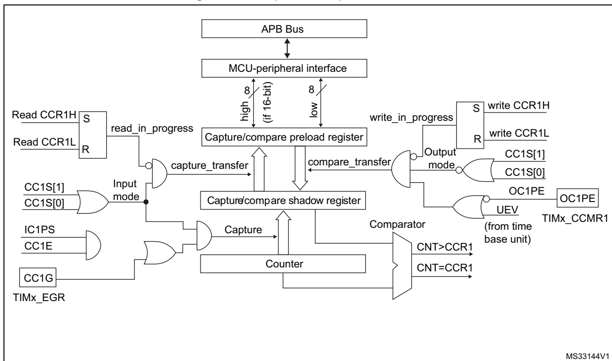
Figure 125. Capture/compare channel 1 main circuit
