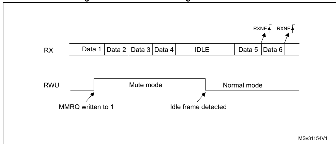
Figure 240. Mute mode using Idle line detection
