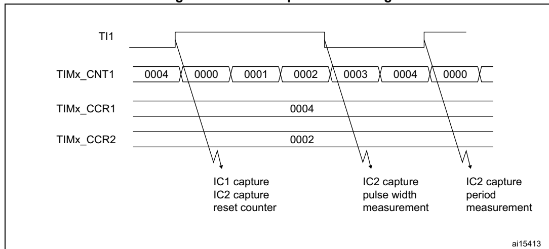
Figure 127. PWM input mode timing
