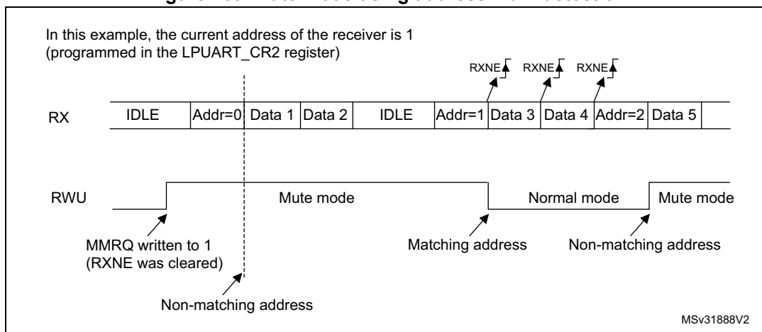
Figure 263. Mute mode using address mark detection
