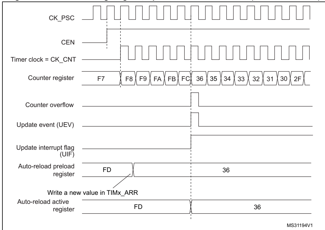
Figure 118. Counter timing diagram, Update event with ARPE=1 (counter overflow)
