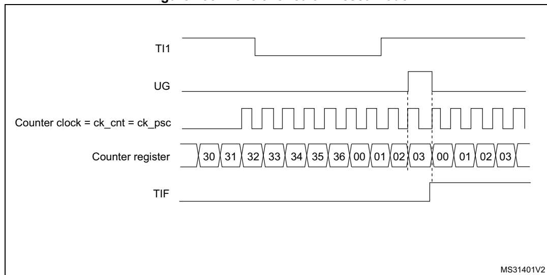
Figure 135. Control circuit in reset mode
