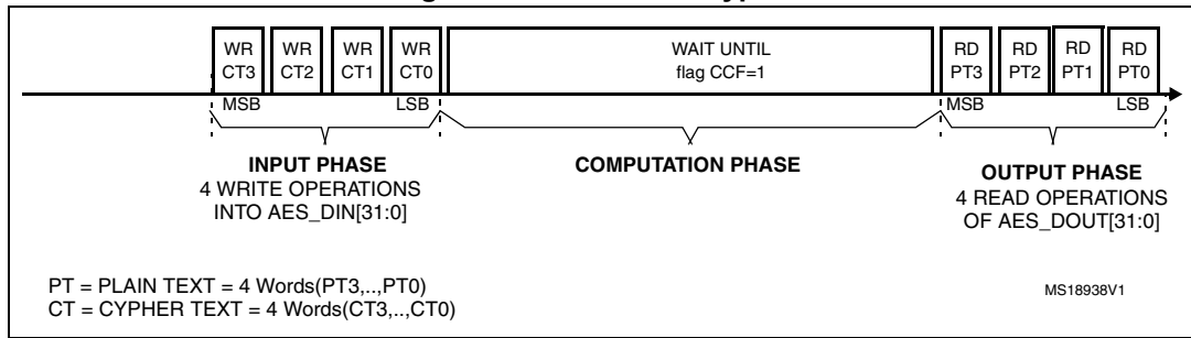
Figure 94. Mode 3: decryption
