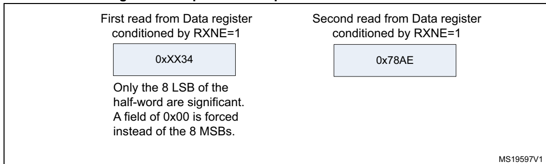
Figure 295. Operations required to receive 0x3478AE
