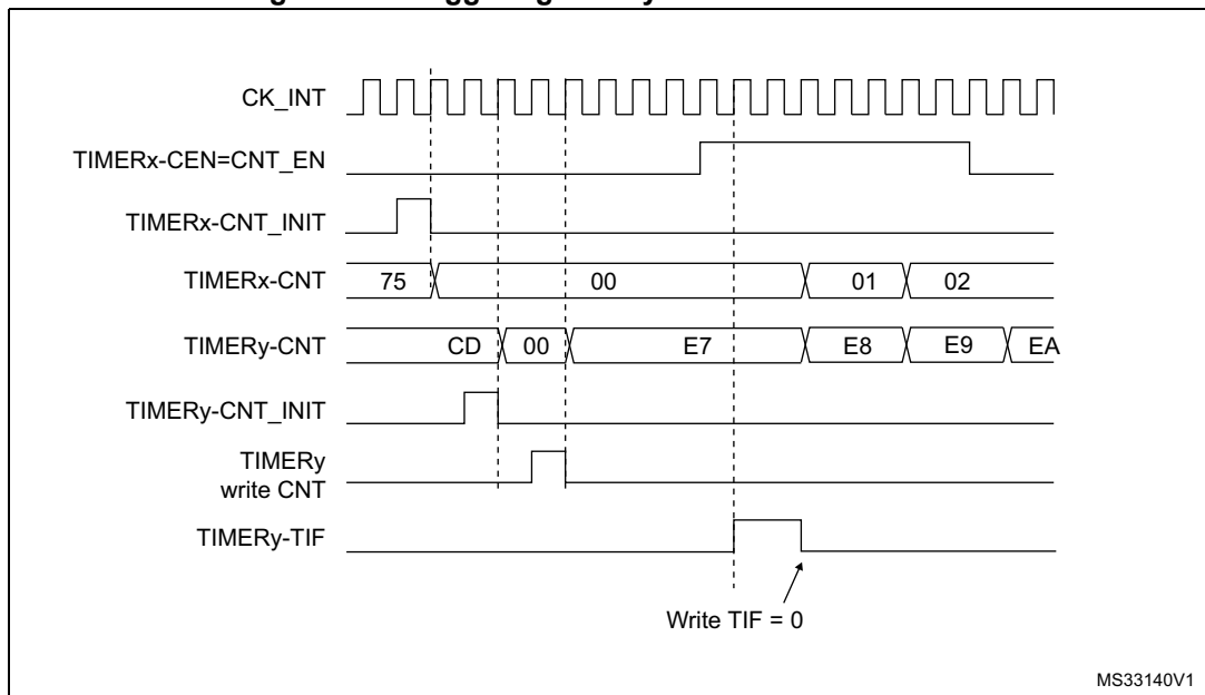
Figure 143. Triggering timer y with Enable of timer x
