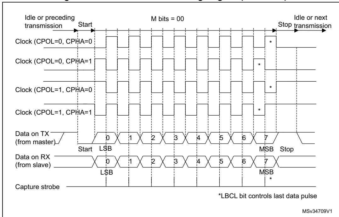
Figure 245. USART data clock timing diagram (M bits = 00)
