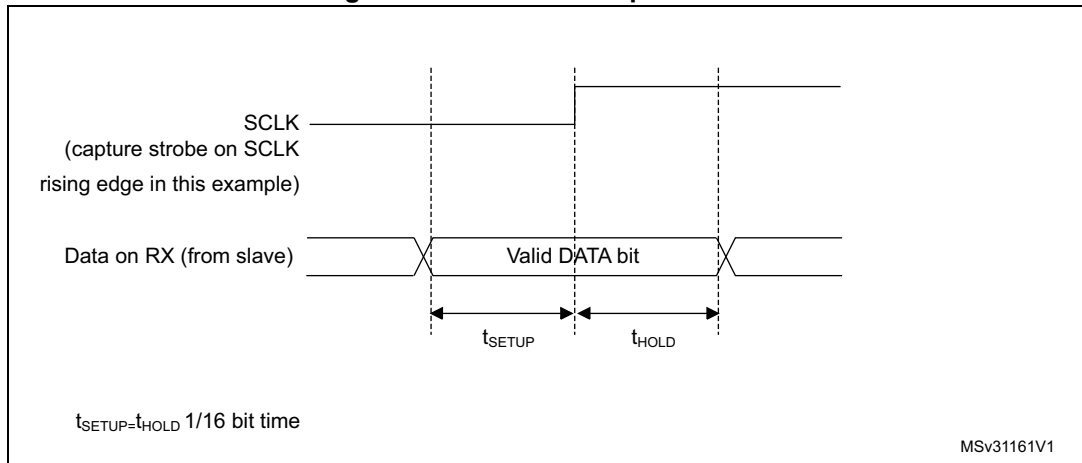
Figure 247. RX data setup/hold time
