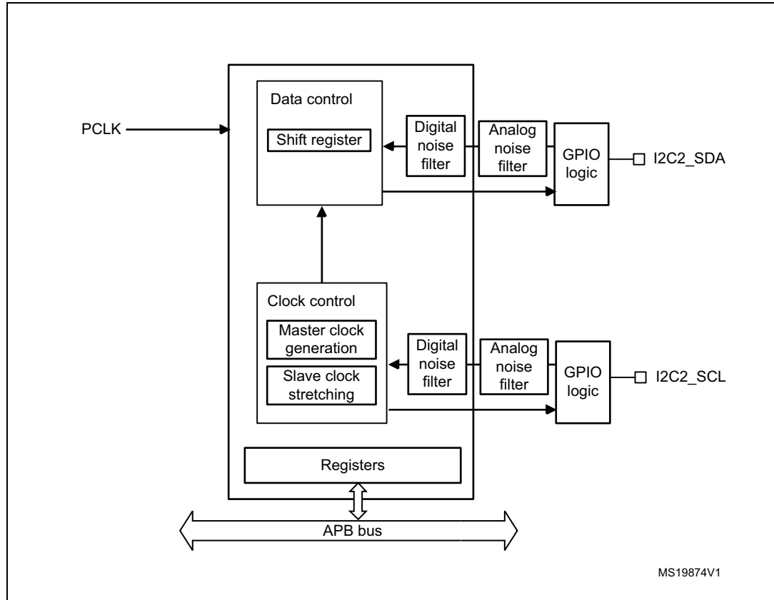
Figure 202. I2C2 block diagram
