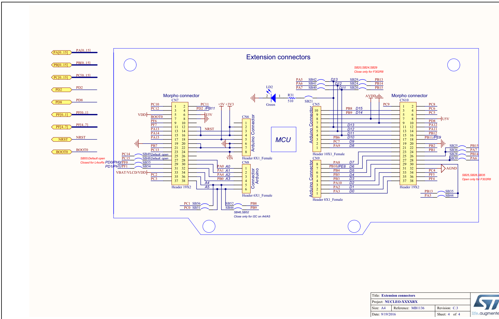
Figure 30. Extension connectors
